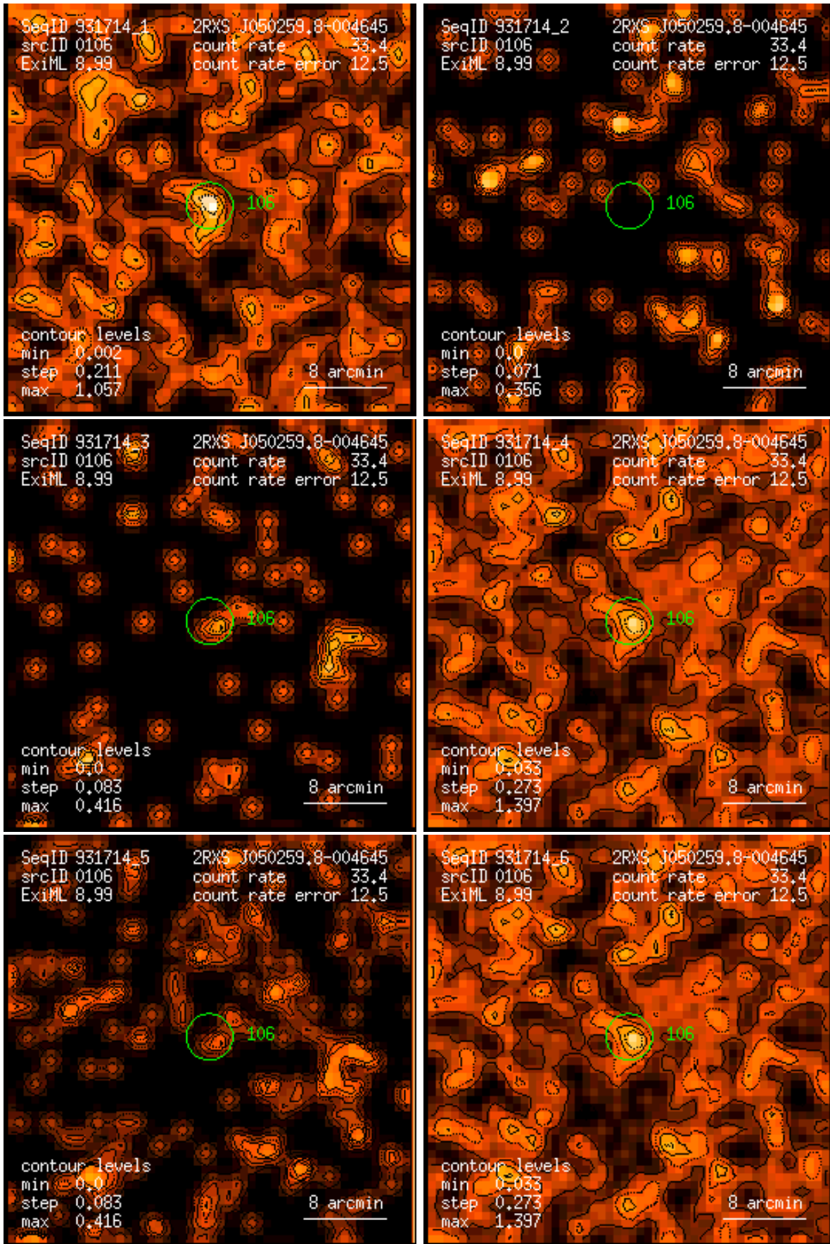
Figure 106: RASS 931714: detection 0106: band rate images, Gaussian filter: (1) PSPC channels 11 – 41, (2) 52 – 90, (3) 91 – 201, (4) 11 – 235, (5) 52 – 201, (6) 11 – 201. Broad band rates in counts/ks. Band rate contour levels in counts/ks/arcmin 2 .
