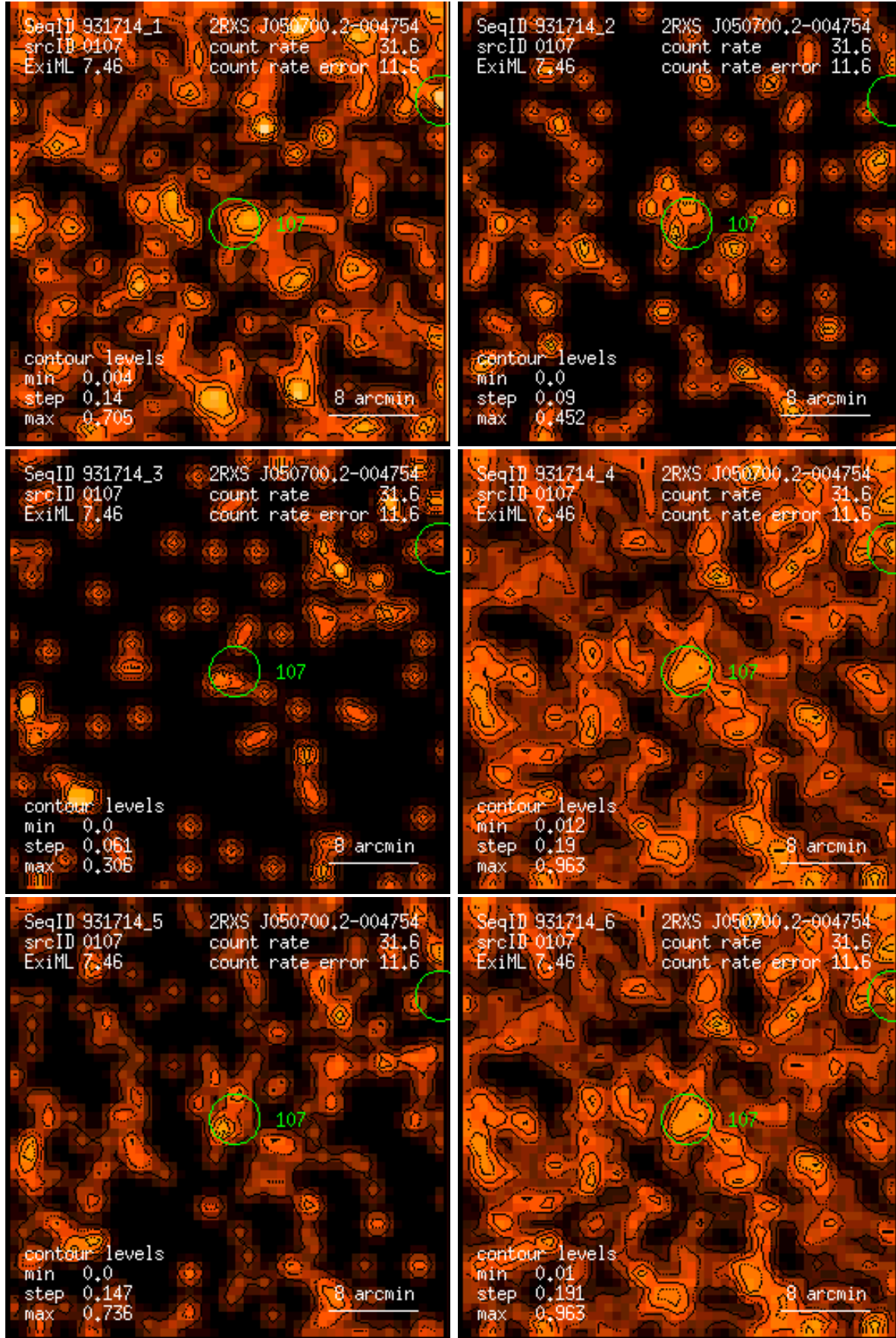
Figure 107: RASS 931714: detection 0107: band rate images, Gaussian filter: (1) PSPC channels 11 – 41, (2) 52 – 90, (3) 91 – 201, (4) 11 – 235, (5) 52 – 201, (6) 11 – 201. Broad band rates in counts/ks. Band rate contour levels in counts/ks/arcmin 2 .
