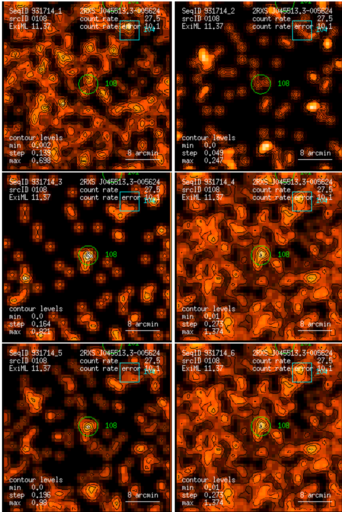
Figure 108: RASS 931714: detection 0108: band rate images, Gaussian filter: (1) PSPC channels 11 – 41, (2) 52 – 90, (3) 91 – 201, (4) 11 – 235, (5) 52 – 201, (6) 11 – 201. Broad band rates in counts/ks. Band rate contour levels in counts/ks/arcmin 2 .
