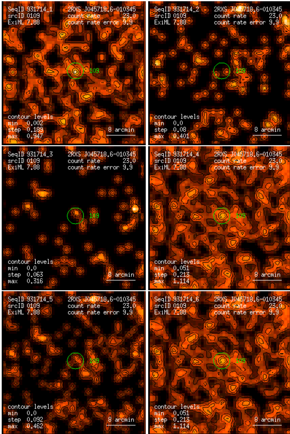
Figure 109: RASS 931714: detection 0109: band rate images, Gaussian filter: (1) PSPC channels 11 – 41, (2) 52 – 90, (3) 91 – 201, (4) 11 – 235, (5) 52 – 201, (6) 11 – 201. Broad band rates in counts/ks. Band rate contour levels in counts/ks/arcmin 2 .
