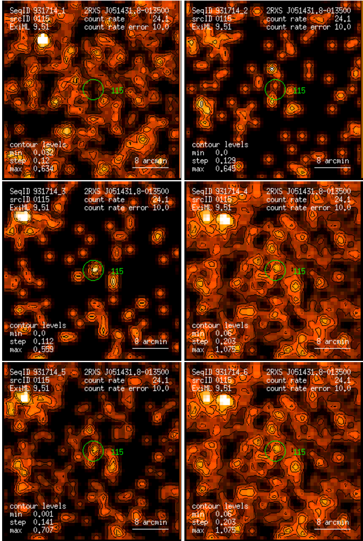
Figure 115: RASS 931714: detection 0115: band rate images, Gaussian filter: (1) PSPC channels 11 – 41, (2) 52 – 90, (3) 91 – 201, (4) 11 – 235, (5) 52 – 201, (6) 11 – 201. Broad band rates in counts/ks. Band rate contour levels in counts/ks/arcmin 2 .
