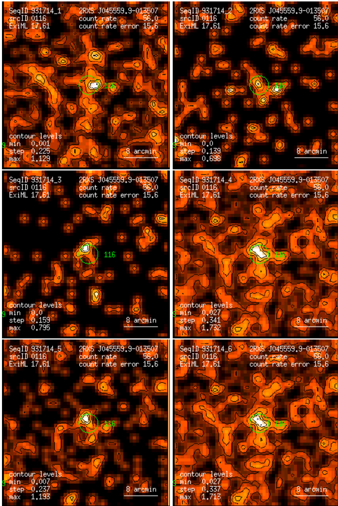
Figure 116: RASS 931714: detection 0116: band rate images, Gaussian filter: (1) PSPC channels 11 – 41, (2) 52 – 90, (3) 91 – 201, (4) 11 – 235, (5) 52 – 201, (6) 11 – 201. Broad band rates in counts/ks. Band rate contour levels in counts/ks/arcmin 2 .
