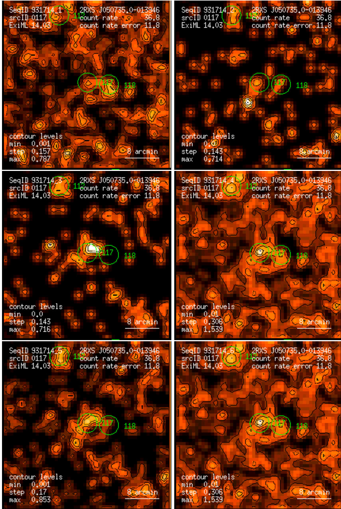
Figure 117: RASS 931714: detection 0117: band rate images, Gaussian filter: (1) PSPC channels 11 – 41, (2) 52 – 90, (3) 91 – 201, (4) 11 – 235, (5) 52 – 201, (6) 11 – 201. Broad band rates in counts/ks. Band rate contour levels in counts/ks/arcmin 2 .
