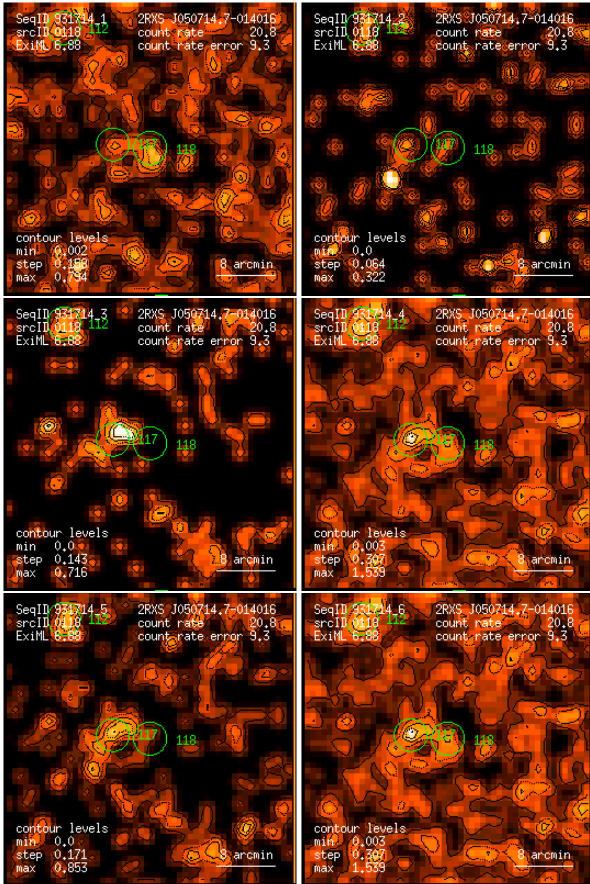
Figure 118: RASS 931714: detection 0118: band rate images, Gaussian filter: (1) PSPC channels 11 – 41, (2) 52 – 90, (3) 91 – 201, (4) 11 – 235, (5) 52 – 201, (6) 11 – 201. Broad band rates in counts/ks. Band rate contour levels in counts/ks/arcmin 2 .
