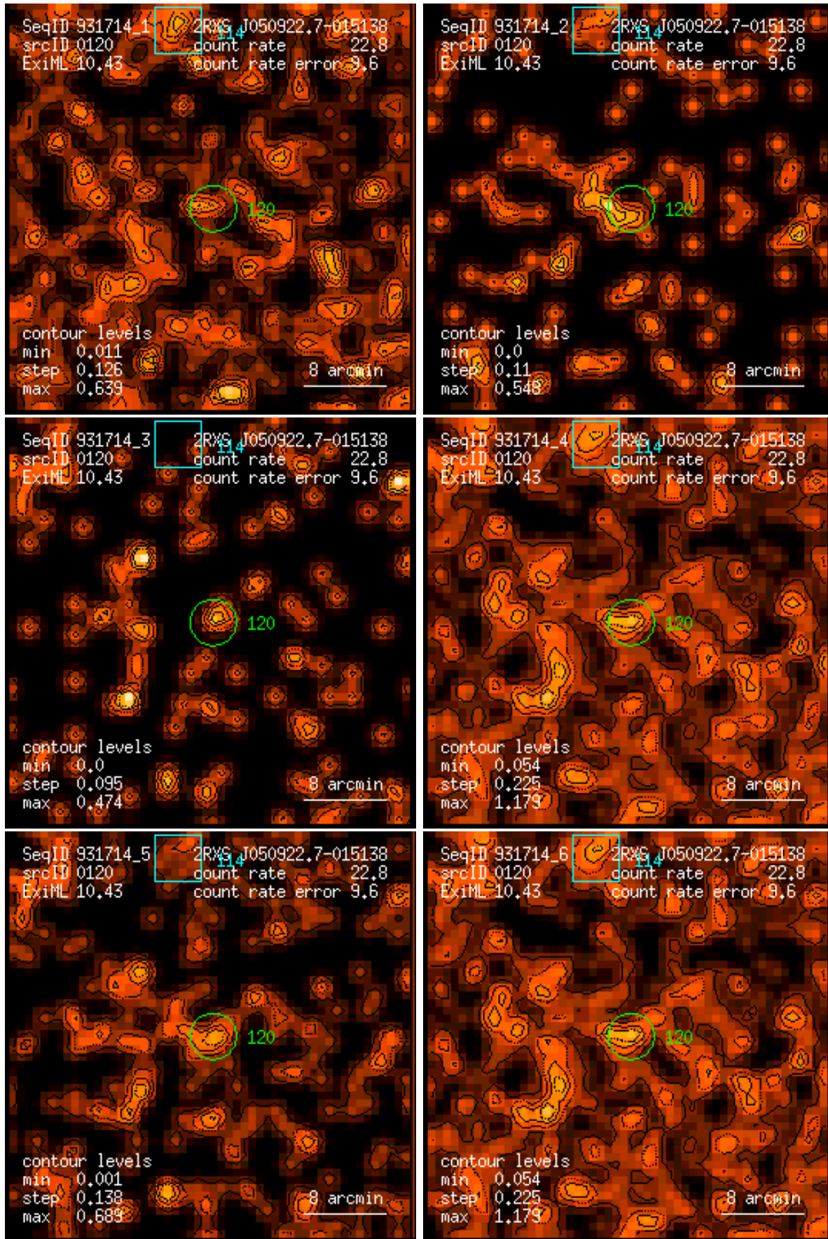
Figure 120: RASS 931714: detection 0120: band rate images, Gaussian filter: (1) PSPC channels 11 – 41, (2) 52 – 90, (3) 91 – 201, (4) 11 – 235, (5) 52 – 201, (6) 11 – 201. Broad band rates in counts/ks. Band rate contour levels in counts/ks/arcmin 2 .
