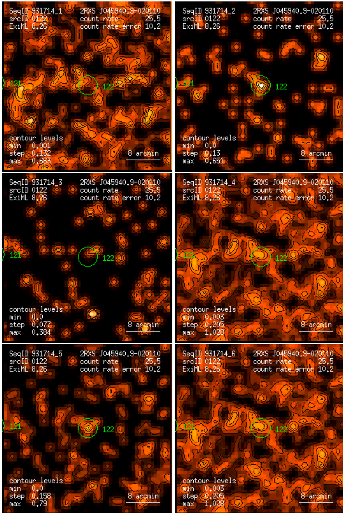
Figure 122: RASS 931714: detection 0122: band rate images, Gaussian filter: (1) PSPC channels 11 – 41, (2) 52 – 90, (3) 91 – 201, (4) 11 – 235, (5) 52 – 201, (6) 11 – 201. Broad band rates in counts/ks. Band rate contour levels in counts/ks/arcmin 2 .
