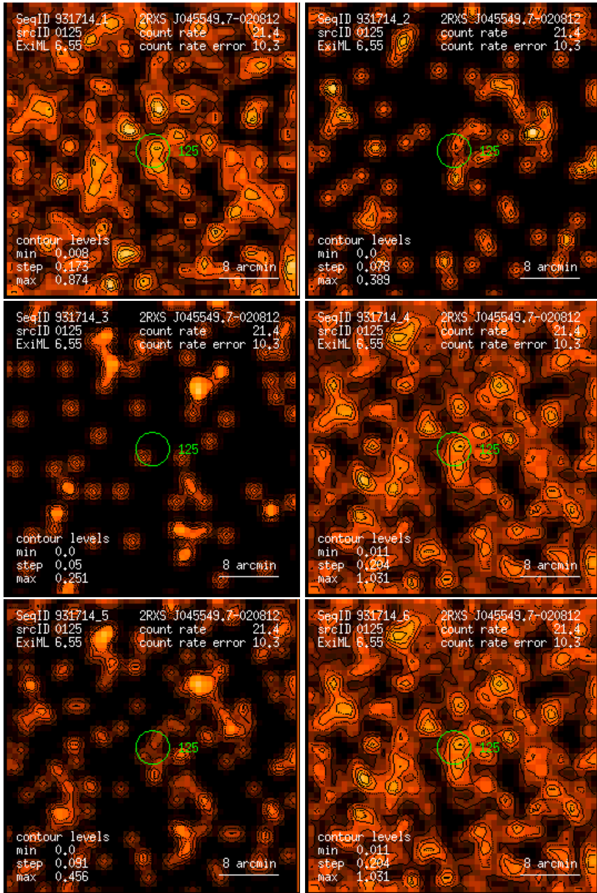
Figure 125: RASS 931714: detection 0125: band rate images, Gaussian filter: (1) PSPC channels 11 – 41, (2) 52 – 90, (3) 91 – 201, (4) 11 – 235, (5) 52 – 201, (6) 11 – 201. Broad band rates in counts/ks. Band rate contour levels in counts/ks/arcmin 2 .
