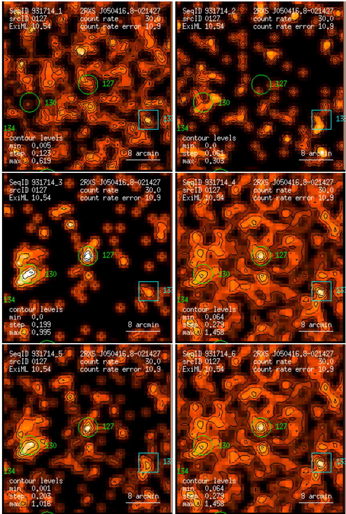
Figure 127: RASS 931714: detection 0127: band rate images, Gaussian filter: (1) PSPC channels 11 – 41, (2) 52 – 90, (3) 91 – 201, (4) 11 – 235, (5) 52 – 201, (6) 11 – 201. Broad band rates in counts/ks. Band rate contour levels in counts/ks/arcmin 2 .
