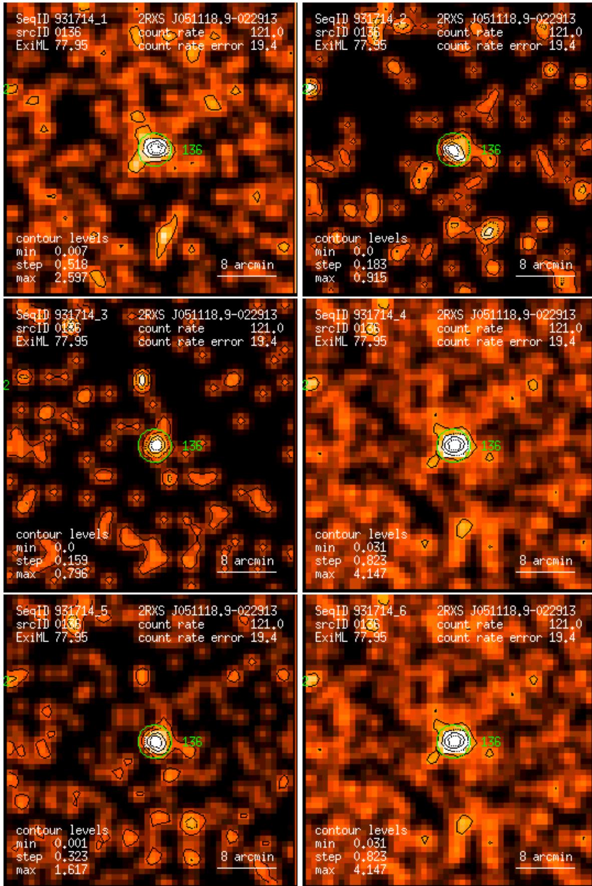
Figure 136: RASS 931714: detection 0136: band rate images, Gaussian filter: (1) PSPC channels 11 – 41, (2) 52 – 90, (3) 91 – 201, (4) 11 – 235, (5) 52 – 201, (6) 11 – 201. Broad band rates in counts/ks. Band rate contour levels in counts/ks/arcmin 2 .
