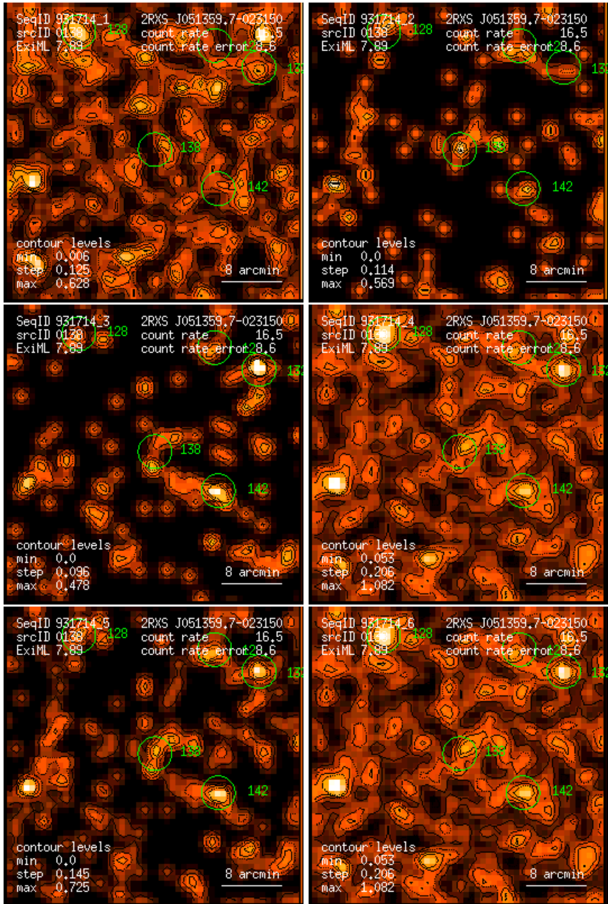
Figure 138: RASS 931714: detection 0138: band rate images, Gaussian filter: (1) PSPC channels 11 – 41, (2) 52 – 90, (3) 91 – 201, (4) 11 – 235, (5) 52 – 201, (6) 11 – 201. Broad band rates in counts/ks. Band rate contour levels in counts/ks/arcmin 2 .
