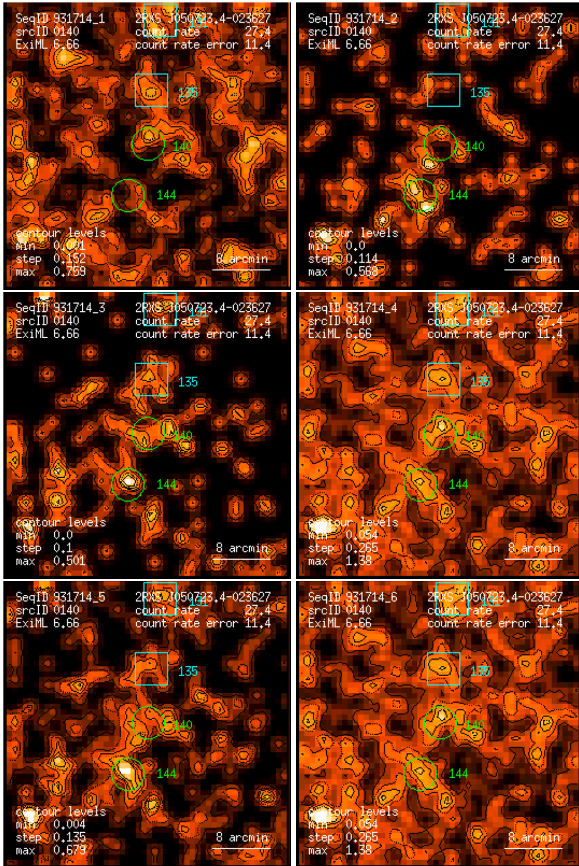
Figure 140: RASS 931714: detection 0140: band rate images, Gaussian filter: (1) PSPC channels 11 – 41, (2) 52 – 90, (3) 91 – 201, (4) 11 – 235, (5) 52 – 201, (6) 11 – 201. Broad band rates in counts/ks. Band rate contour levels in counts/ks/arcmin 2 .
