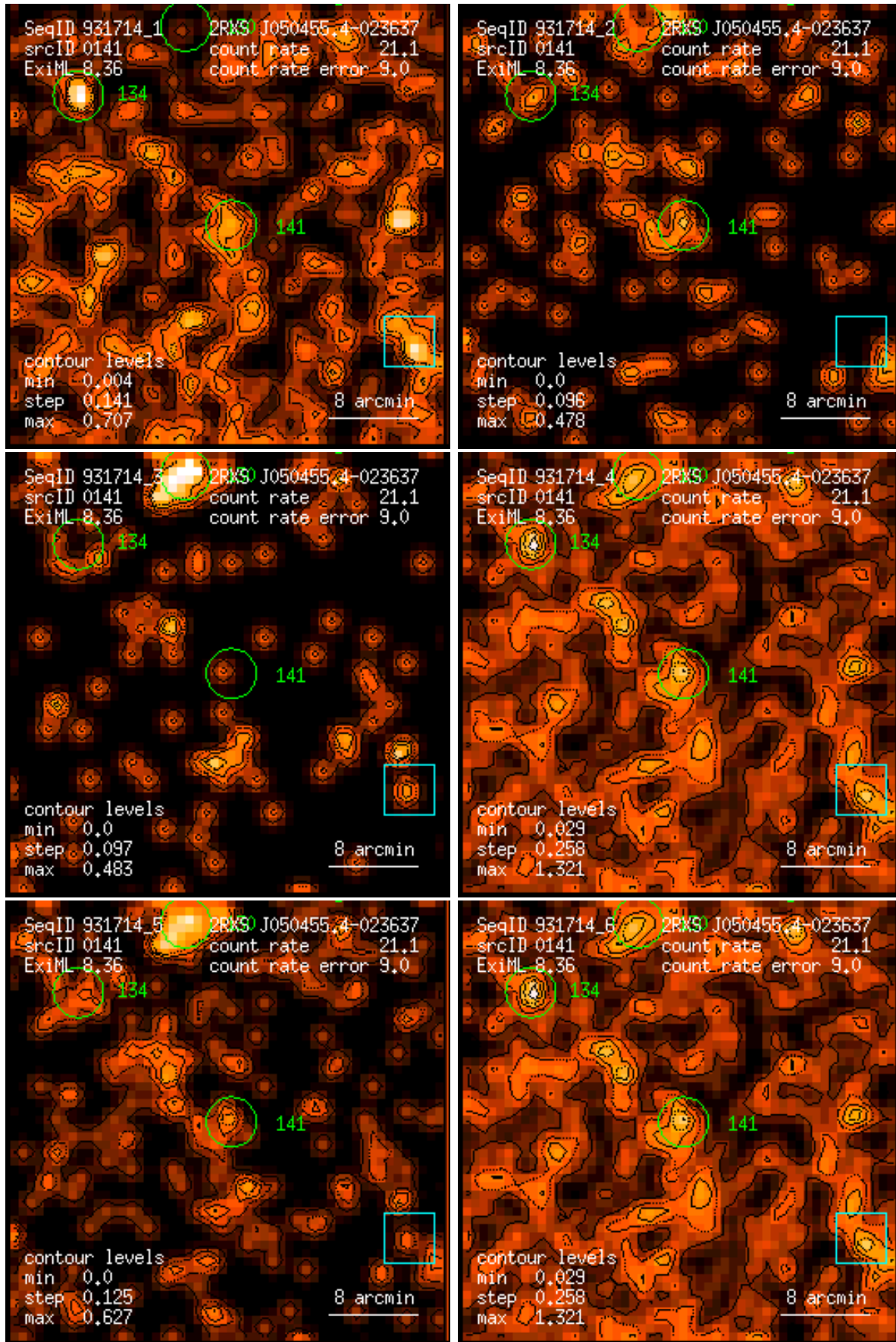
Figure 141: RASS 931714: detection 0141: band rate images, Gaussian filter: (1) PSPC channels 11 – 41, (2) 52 – 90, (3) 91 – 201, (4) 11 – 235, (5) 52 – 201, (6) 11 – 201. Broad band rates in counts/ks. Band rate contour levels in counts/ks/arcmin 2 .
