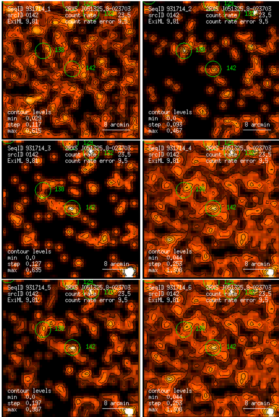
Figure 142: RASS 931714: detection 0142: band rate images, Gaussian filter: (1) PSPC channels 11 – 41, (2) 52 – 90, (3) 91 – 201, (4) 11 – 235, (5) 52 – 201, (6) 11 – 201. Broad band rates in counts/ks. Band rate contour levels in counts/ks/arcmin 2 .
