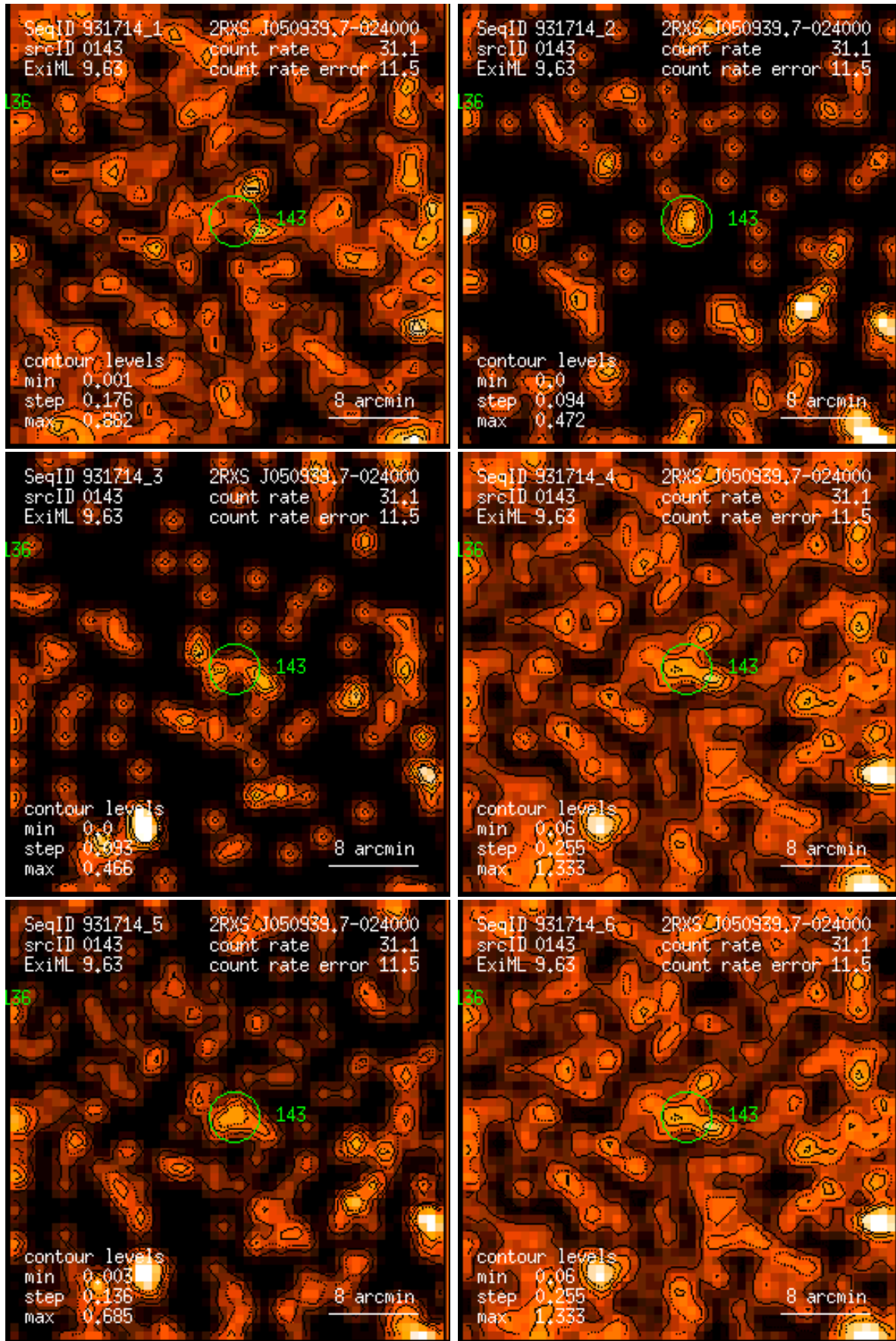
Figure 143: RASS 931714: detection 0143: band rate images, Gaussian filter: (1) PSPC channels 11 – 41, (2) 52 – 90, (3) 91 – 201, (4) 11 – 235, (5) 52 – 201, (6) 11 – 201. Broad band rates in counts/ks. Band rate contour levels in counts/ks/arcmin 2 .
