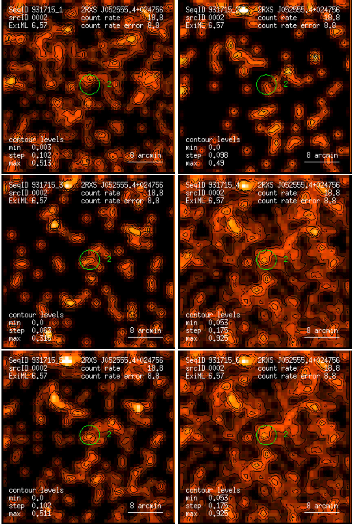
Figure 2: RASS 931715: detection 0002: band rate images, Gaussian filter: (1) PSPC channels 11 – 41, (2) 52 – 90, (3) 91 – 201, (4) 11 – 235, (5) 52 – 201, (6) 11 – 201. Broad band rates in counts/ks. Band rate contour levels in counts/ks/arcmin 2 .
