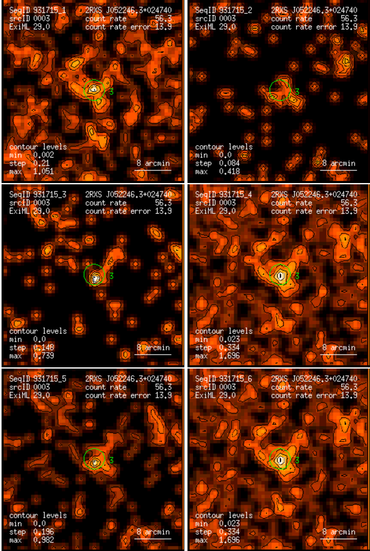
Figure 3: RASS 931715: detection 0003: band rate images, Gaussian filter: (1) PSPC channels 11 – 41, (2) 52 – 90, (3) 91 – 201, (4) 11 – 235, (5) 52 – 201, (6) 11 – 201. Broad band rates in counts/ks. Band rate contour levels in counts/ks/arcmin 2 .
