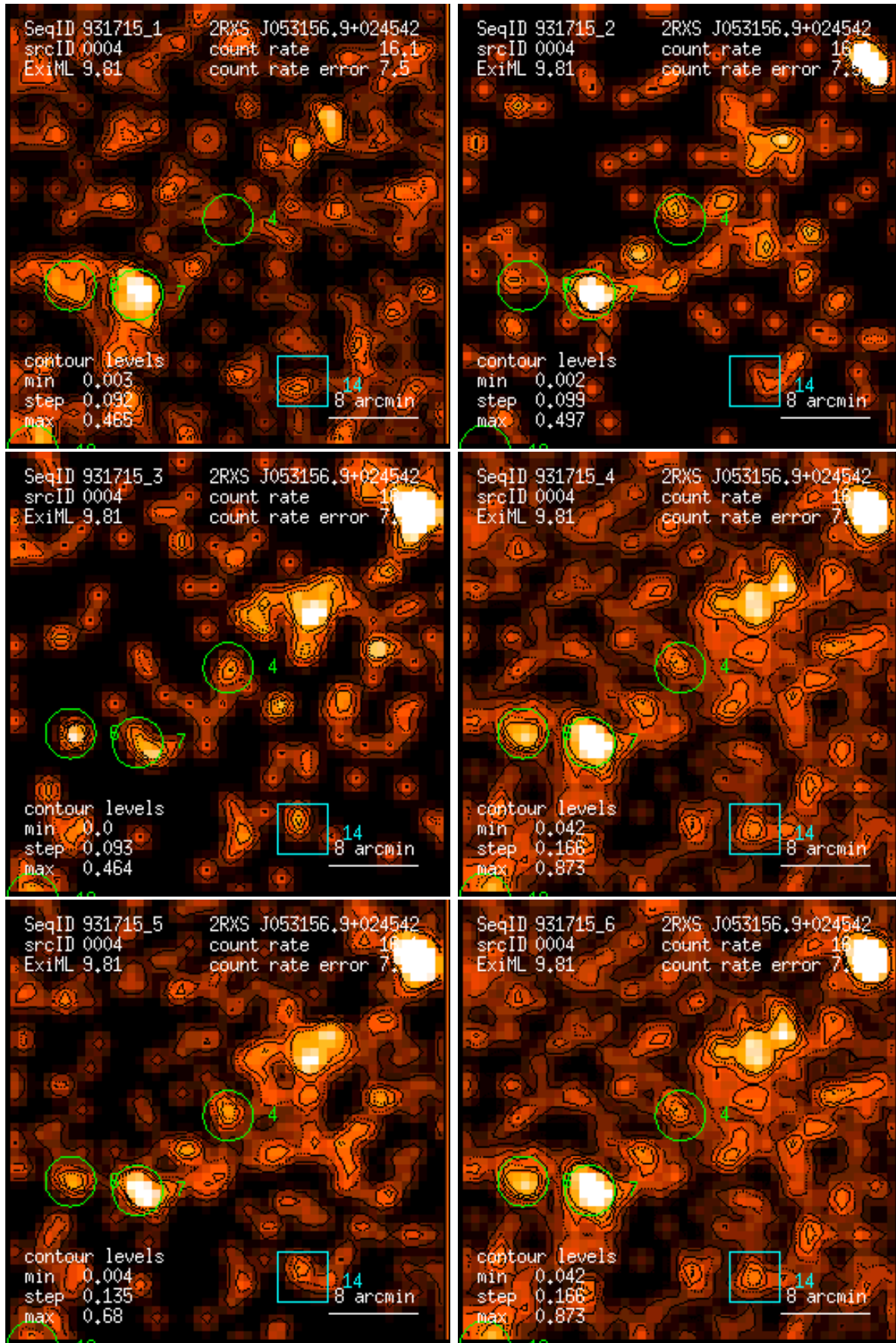
Figure 4: RASS 931715: detection 0004: band rate images, Gaussian filter: (1) PSPC channels 11 – 41, (2) 52 – 90, (3) 91 – 201, (4) 11 – 235, (5) 52 – 201, (6) 11 – 201. Broad band rates in counts/ks. Band rate contour levels in counts/ks/arcmin 2 .
