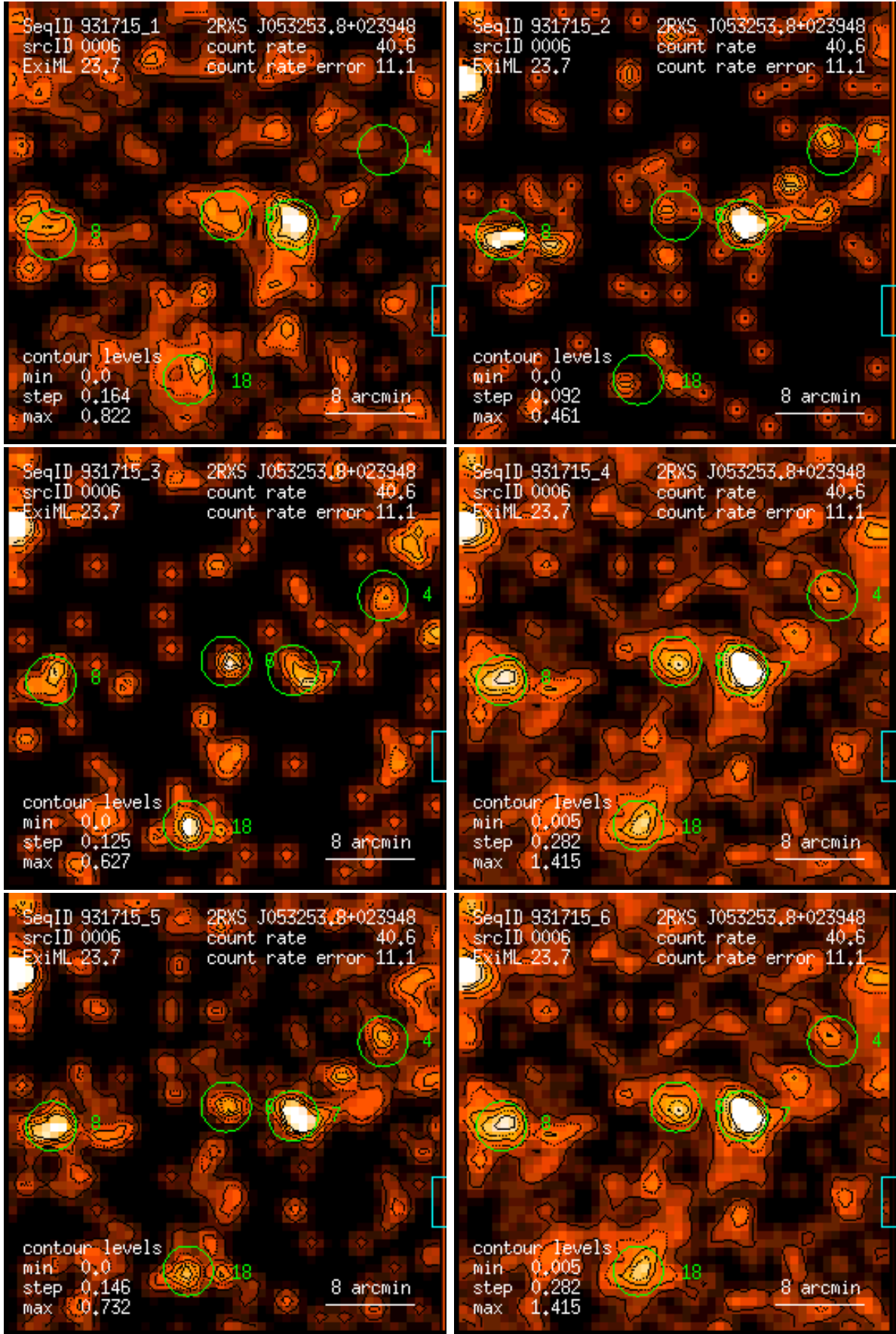
Figure 6: RASS 931715: detection 0006: band rate images, Gaussian filter: (1) PSPC channels 11 – 41, (2) 52 – 90, (3) 91 – 201, (4) 11 – 235, (5) 52 – 201, (6) 11 – 201. Broad band rates in counts/ks. Band rate contour levels in counts/ks/arcmin 2 .
