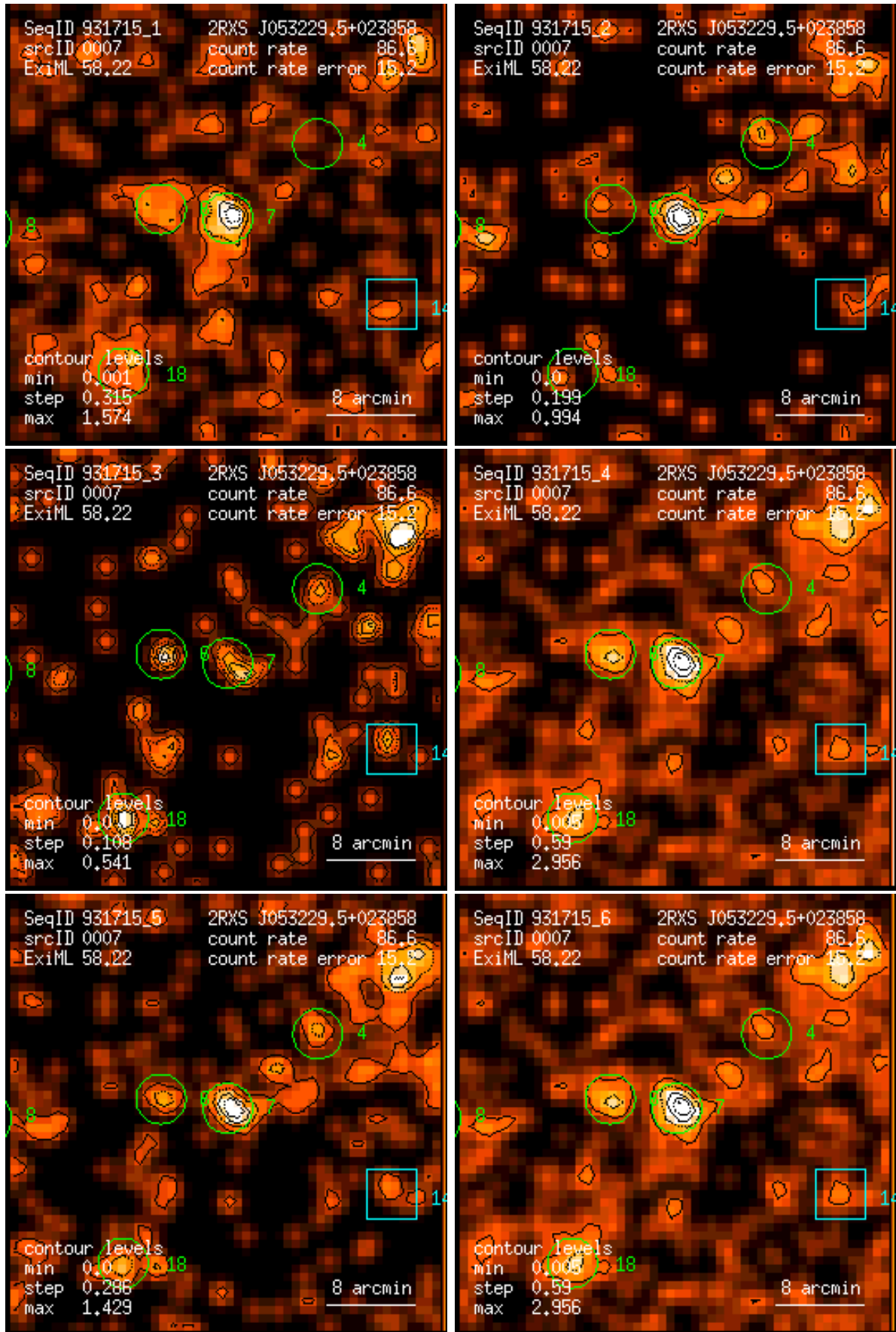
Figure 7: RASS 931715: detection 0007: band rate images, Gaussian filter: (1) PSPC channels 11 – 41, (2) 52 – 90, (3) 91 – 201, (4) 11 – 235, (5) 52 – 201, (6) 11 – 201. Broad band rates in counts/ks. Band rate contour levels in counts/ks/arcmin 2 .
