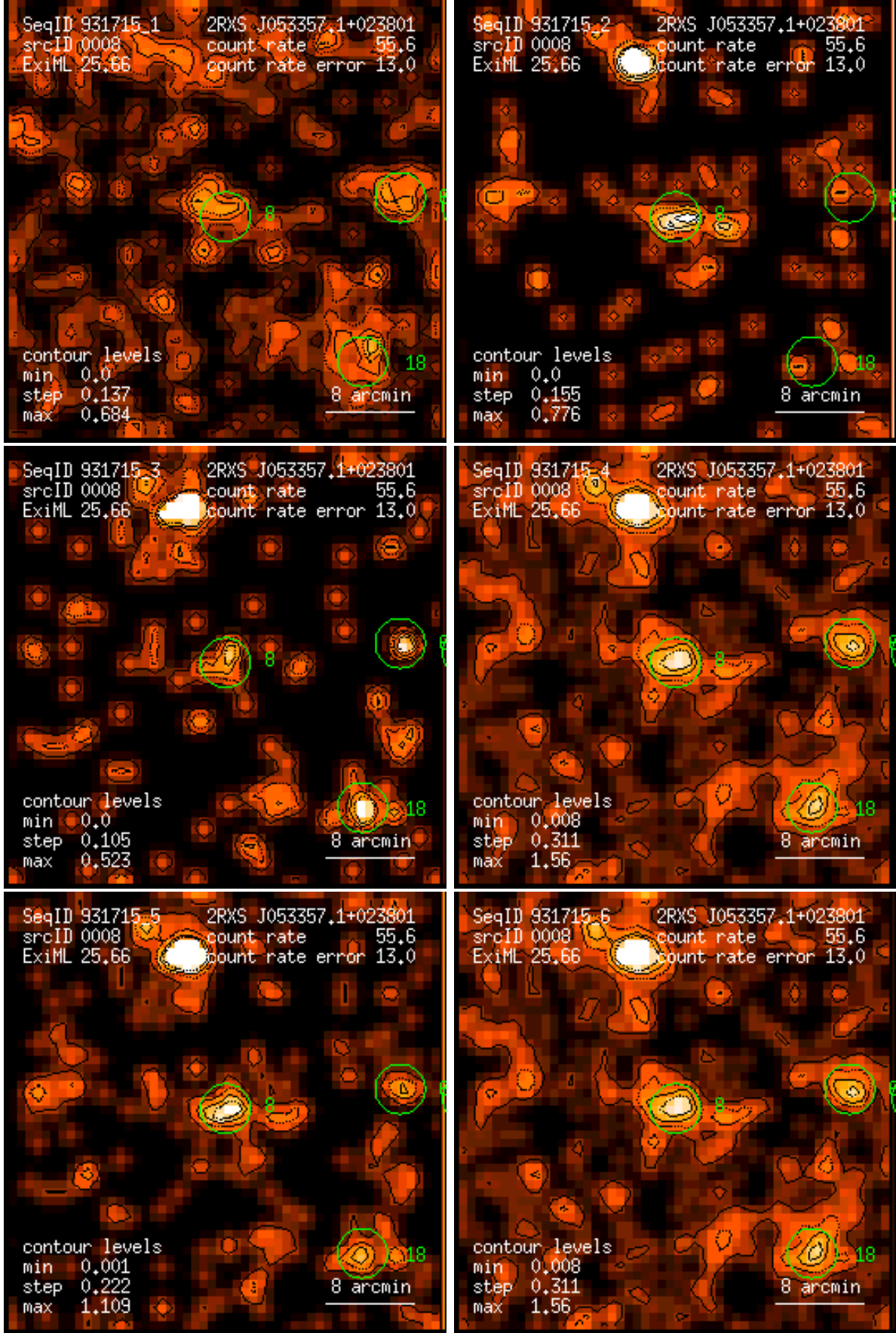
Figure 8: RASS 931715: detection 0008: band rate images, Gaussian filter: (1) PSPC channels 11 – 41, (2) 52 – 90, (3) 91 – 201, (4) 11 – 235, (5) 52 – 201, (6) 11 – 201. Broad band rates in counts/ks. Band rate contour levels in counts/ks/arcmin 2 .
