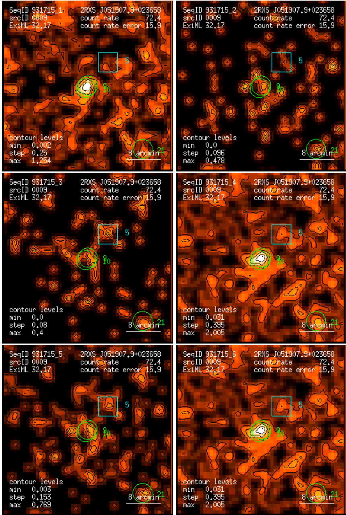
Figure 9: RASS 931715: detection 0009: band rate images, Gaussian filter: (1) PSPC channels 11 – 41, (2) 52 – 90, (3) 91 – 201, (4) 11 – 235, (5) 52 – 201, (6) 11 – 201. Broad band rates in counts/ks. Band rate contour levels in counts/ks/arcmin 2 .
