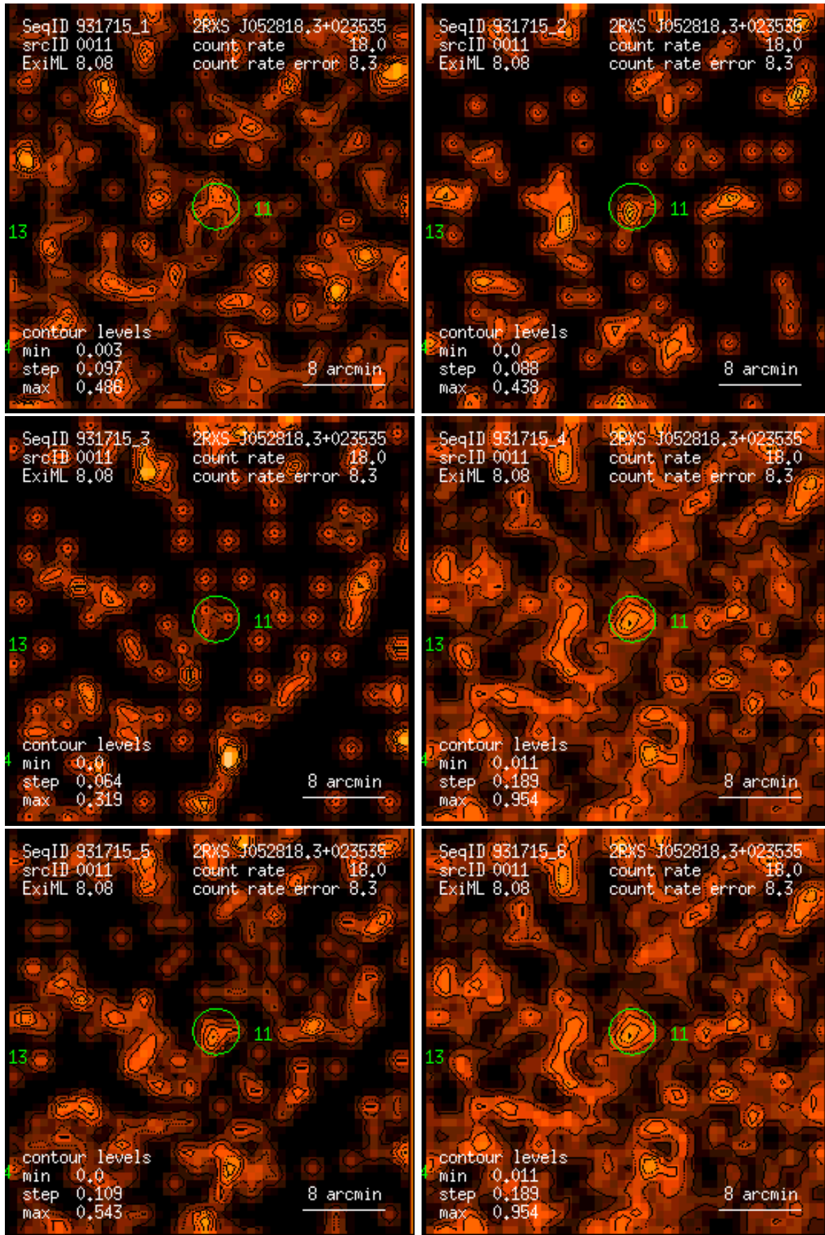
Figure 11: RASS 931715: detection 0011: band rate images, Gaussian filter: (1) PSPC channels 11 – 41, (2) 52 – 90, (3) 91 – 201, (4) 11 – 235, (5) 52 – 201, (6) 11 – 201. Broad band rates in counts/ks. Band rate contour levels in counts/ks/arcmin 2 .
