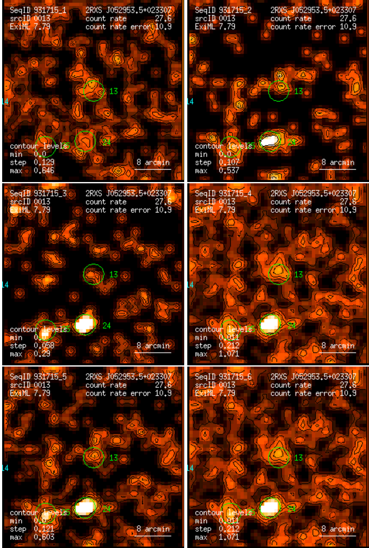
Figure 13: RASS 931715: detection 0013: band rate images, Gaussian filter: (1) PSPC channels 11 – 41, (2) 52 – 90, (3) 91 – 201, (4) 11 – 235, (5) 52 – 201, (6) 11 – 201. Broad band rates in counts/ks. Band rate contour levels in counts/ks/arcmin 2 .
