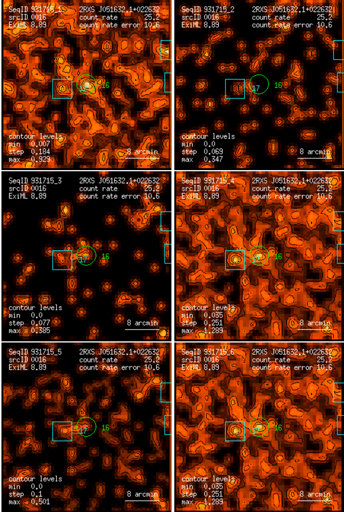
Figure 16: RASS 931715: detection 0016: band rate images, Gaussian filter: (1) PSPC channels 11 – 41, (2) 52 – 90, (3) 91 – 201, (4) 11 – 235, (5) 52 – 201, (6) 11 – 201. Broad band rates in counts/ks. Band rate contour levels in counts/ks/arcmin 2 .
