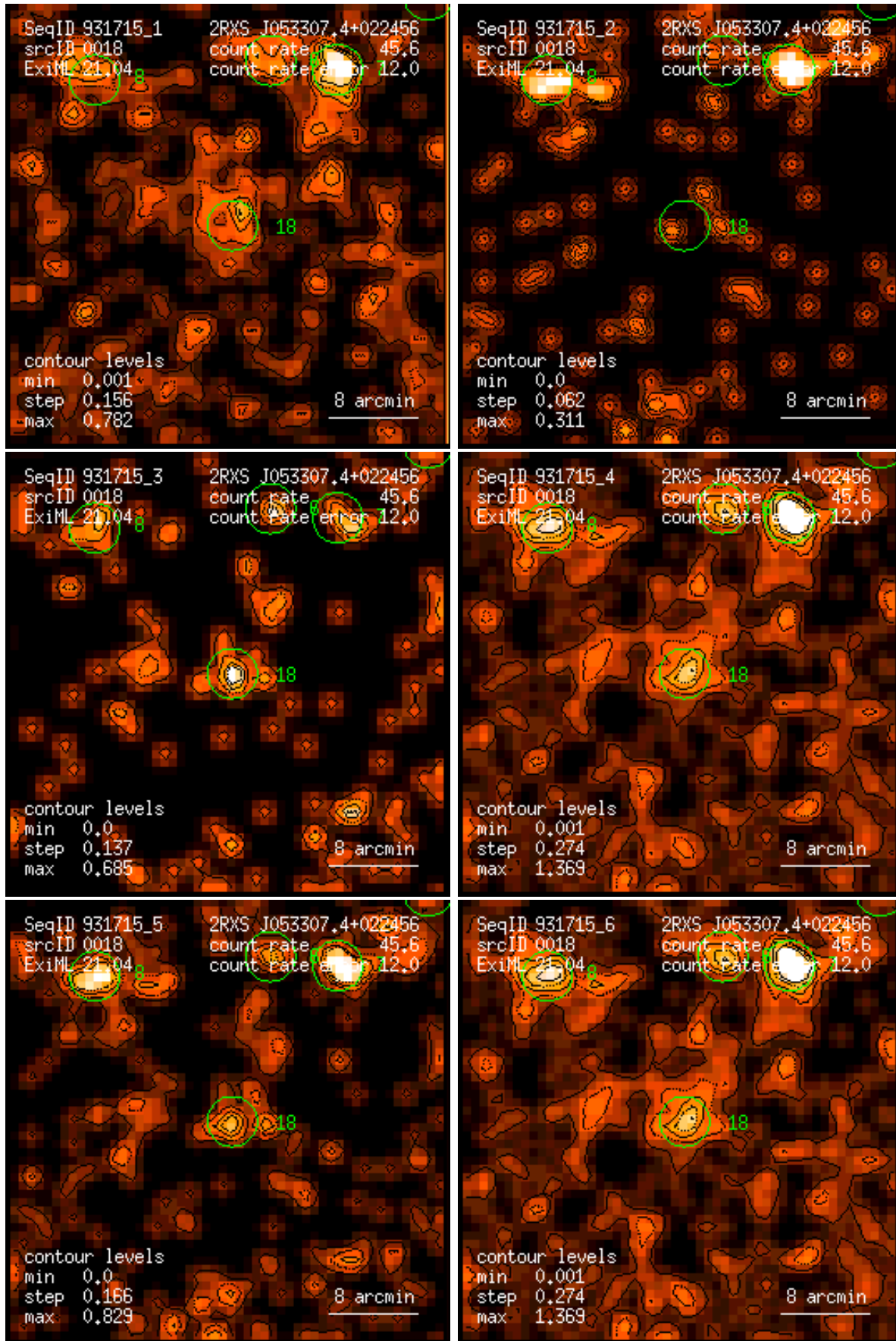
Figure 18: RASS 931715: detection 0018: band rate images, Gaussian filter: (1) PSPC channels 11 – 41, (2) 52 – 90, (3) 91 – 201, (4) 11 – 235, (5) 52 – 201, (6) 11 – 201. Broad band rates in counts/ks. Band rate contour levels in counts/ks/arcmin 2 .
