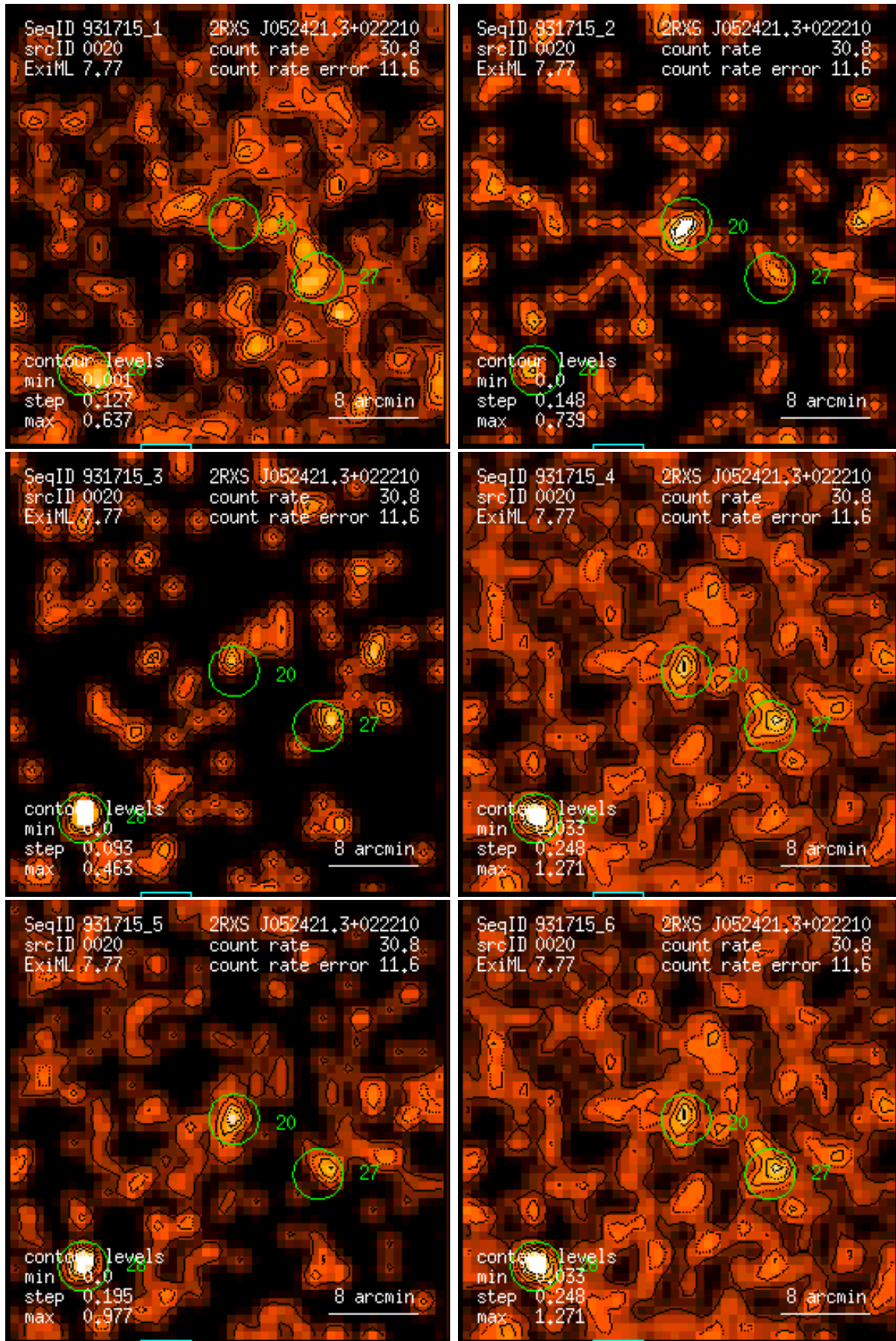
Figure 20: RASS 931715: detection 0020: band rate images, Gaussian filter: (1) PSPC channels 11 – 41, (2) 52 – 90, (3) 91 – 201, (4) 11 – 235, (5) 52 – 201, (6) 11 – 201. Broad band rates in counts/ks. Band rate contour levels in counts/ks/arcmin 2 .
