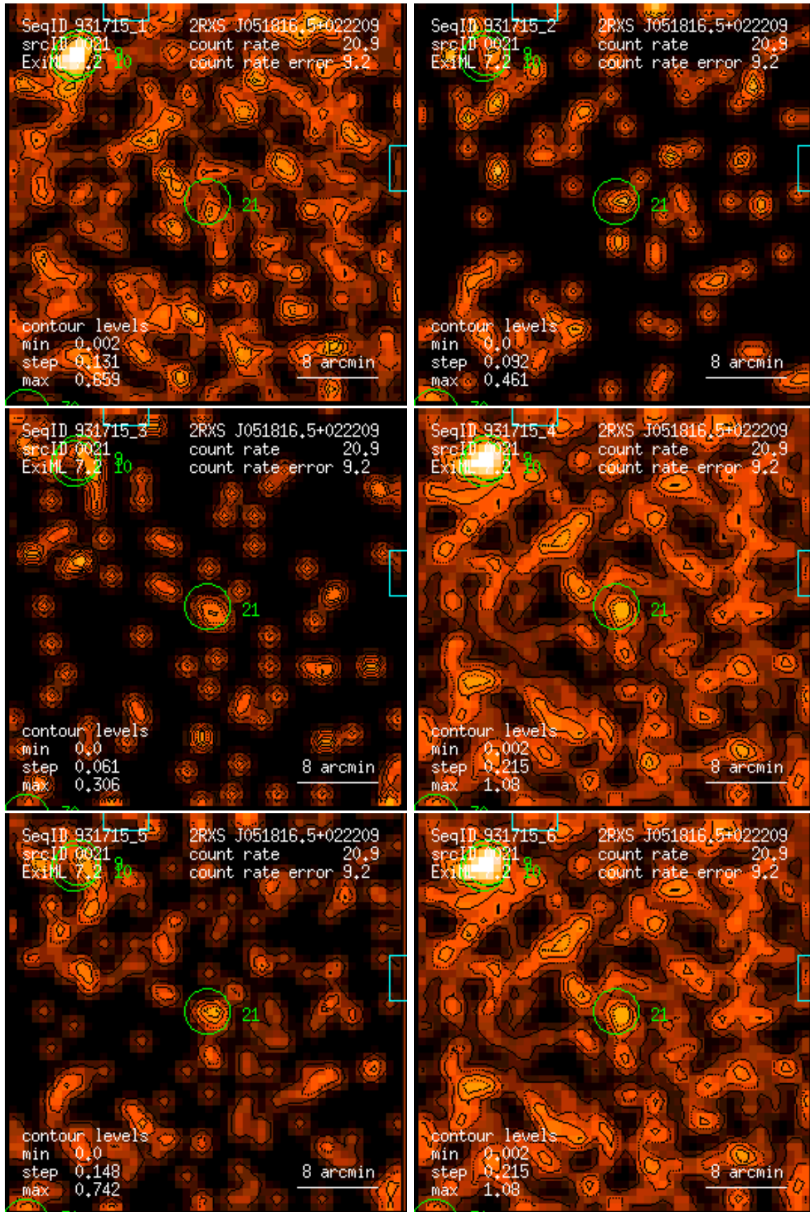
Figure 21: RASS 931715: detection 0021: band rate images, Gaussian filter: (1) PSPC channels 11 – 41, (2) 52 – 90, (3) 91 – 201, (4) 11 – 235, (5) 52 – 201, (6) 11 – 201. Broad band rates in counts/ks. Band rate contour levels in counts/ks/arcmin 2 .
