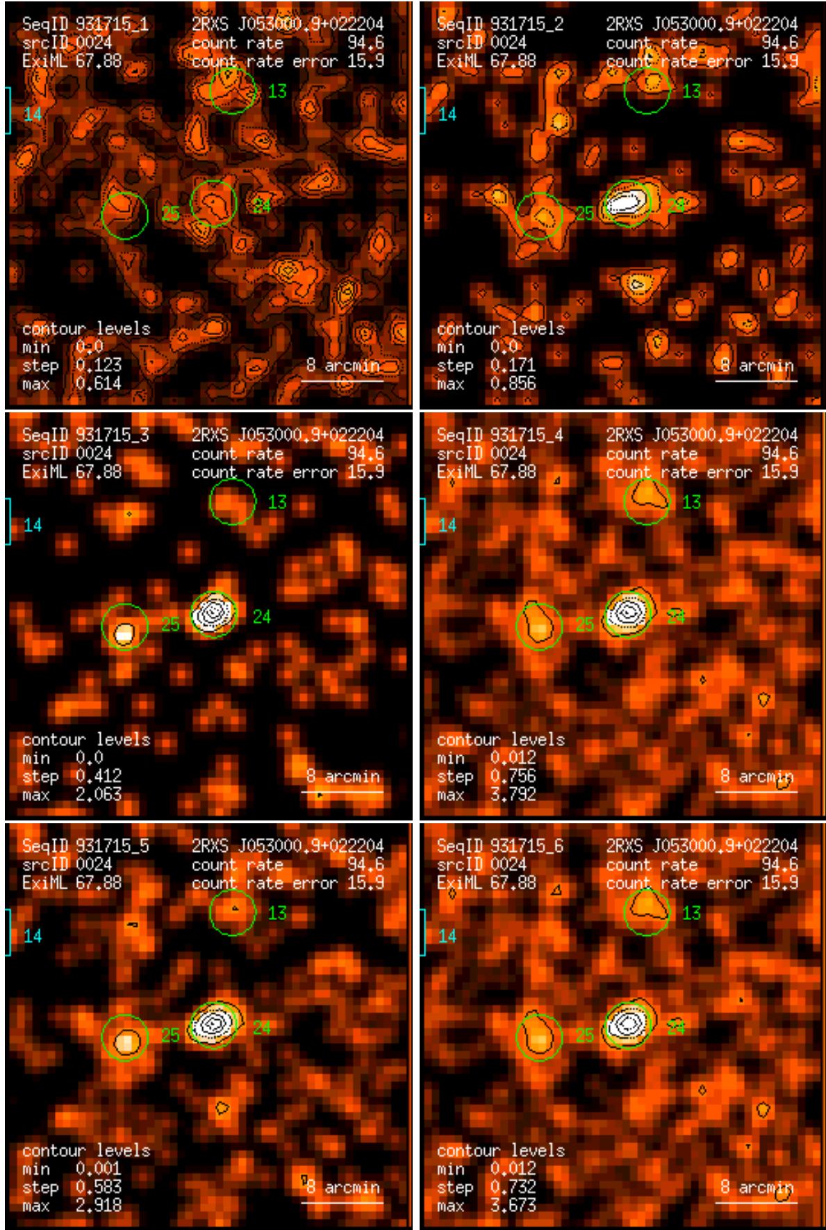
Figure 24: RASS 931715: detection 0024: band rate images, Gaussian filter: (1) PSPC channels 11 – 41, (2) 52 – 90, (3) 91 – 201, (4) 11 – 235, (5) 52 – 201, (6) 11 – 201. Broad band rates in counts/ks. Band rate contour levels in counts/ks/arcmin 2 .
