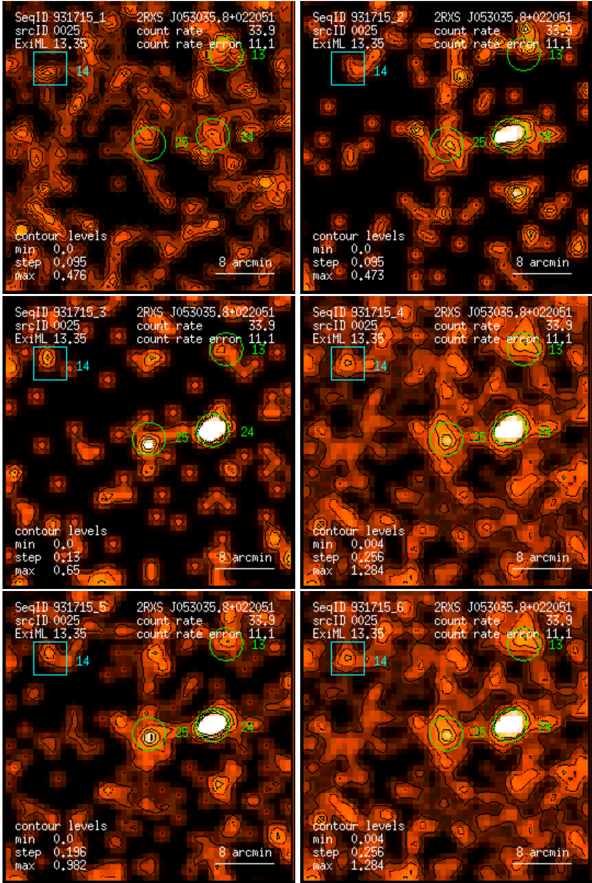
Figure 25: RASS 931715: detection 0025: band rate images, Gaussian filter: (1) PSPC channels 11 – 41, (2) 52 – 90, (3) 91 – 201, (4) 11 – 235, (5) 52 – 201, (6) 11 – 201. Broad band rates in counts/ks. Band rate contour levels in counts/ks/arcmin 2 .
