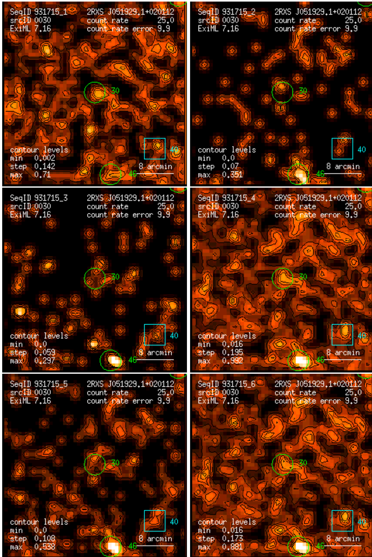
Figure 30: RASS 931715: detection 0030: band rate images, Gaussian filter: (1) PSPC channels 11 – 41, (2) 52 – 90, (3) 91 – 201, (4) 11 – 235, (5) 52 – 201, (6) 11 – 201. Broad band rates in counts/ks. Band rate contour levels in counts/ks/arcmin 2 .
