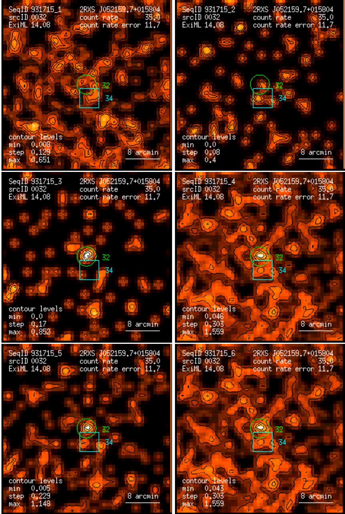
Figure 32: RASS 931715: detection 0032: band rate images, Gaussian filter: (1) PSPC channels 11 – 41, (2) 52 – 90, (3) 91 – 201, (4) 11 – 235, (5) 52 – 201, (6) 11 – 201. Broad band rates in counts/ks. Band rate contour levels in counts/ks/arcmin 2 .
