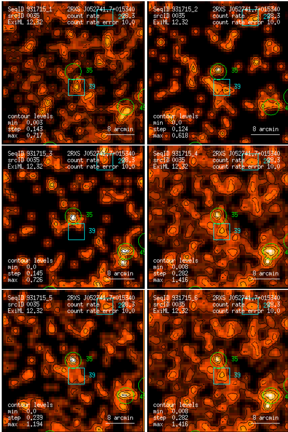
Figure 35: RASS 931715: detection 0035: band rate images, Gaussian filter: (1) PSPC channels 11 – 41, (2) 52 – 90, (3) 91 – 201, (4) 11 – 235, (5) 52 – 201, (6) 11 – 201. Broad band rates in counts/ks. Band rate contour levels in counts/ks/arcmin 2 .
