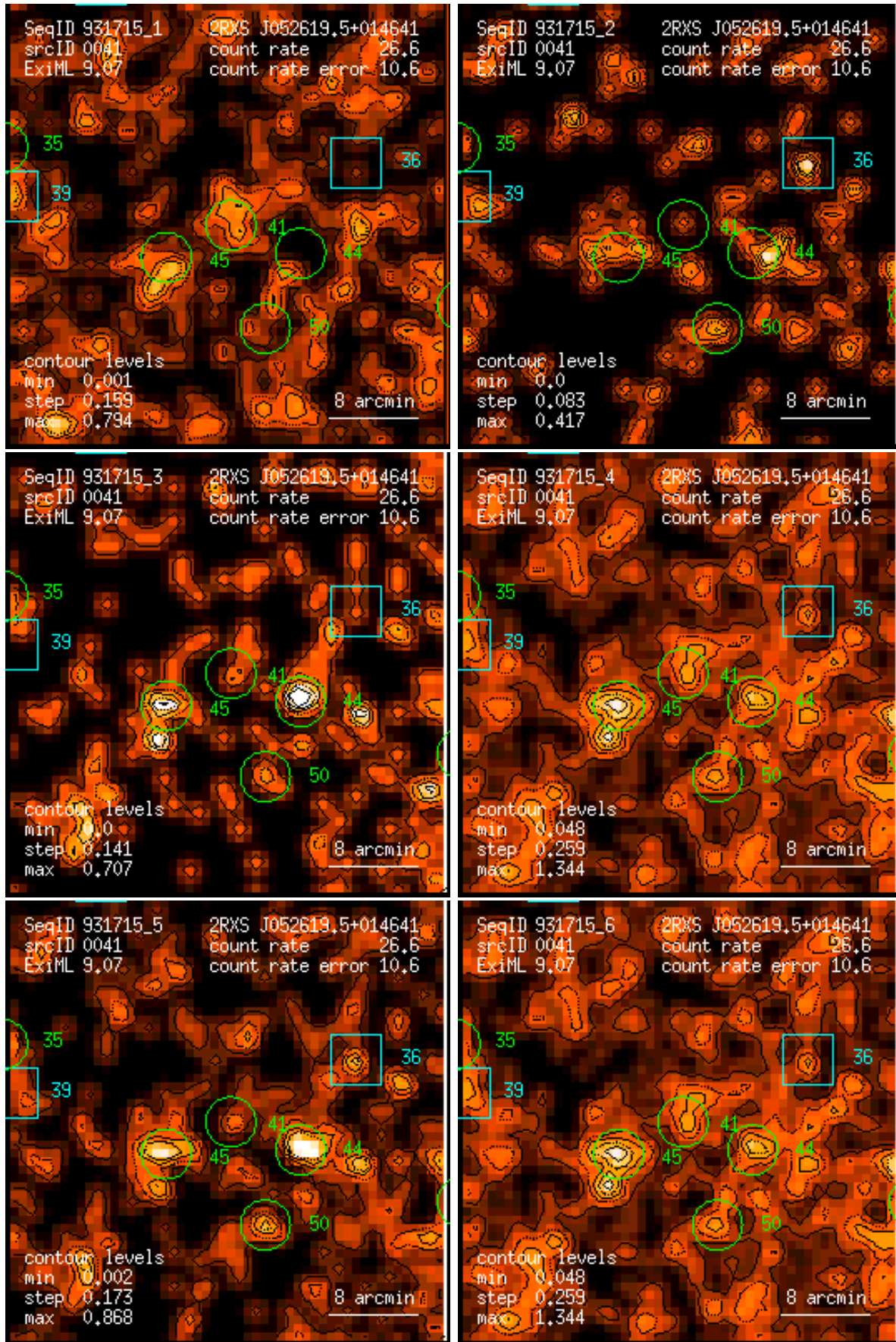
Figure 41: RASS 931715: detection 0041: band rate images, Gaussian filter: (1) PSPC channels 11 – 41, (2) 52 – 90, (3) 91 – 201, (4) 11 – 235, (5) 52 – 201, (6) 11 – 201. Broad band rates in counts/ks. Band rate contour levels in counts/ks/arcmin 2 .
