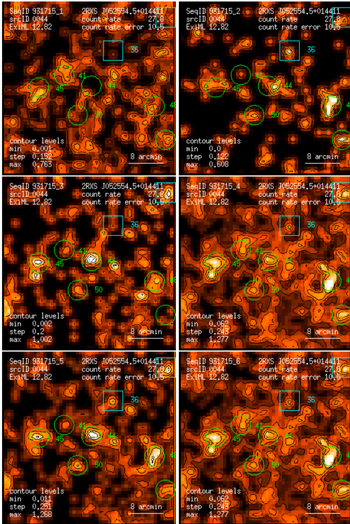
Figure 44: RASS 931715: detection 0044: band rate images, Gaussian filter: (1) PSPC channels 11 – 41, (2) 52 – 90, (3) 91 – 201, (4) 11 – 235, (5) 52 – 201, (6) 11 – 201. Broad band rates in counts/ks. Band rate contour levels in counts/ks/arcmin 2 .
