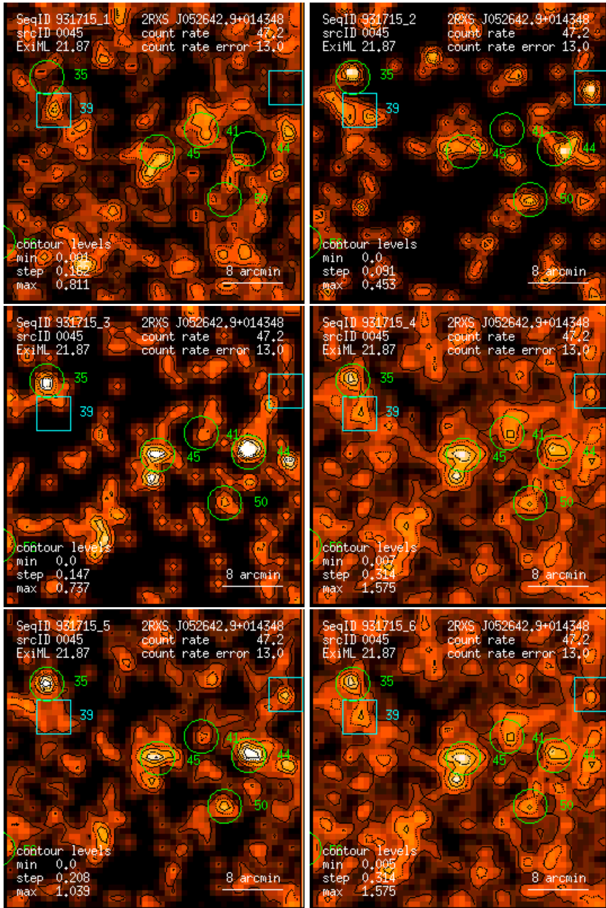
Figure 45: RASS 931715: detection 0045: band rate images, Gaussian filter: (1) PSPC channels 11 – 41, (2) 52 – 90, (3) 91 – 201, (4) 11 – 235, (5) 52 – 201, (6) 11 – 201. Broad band rates in counts/ks. Band rate contour levels in counts/ks/arcmin 2 .
