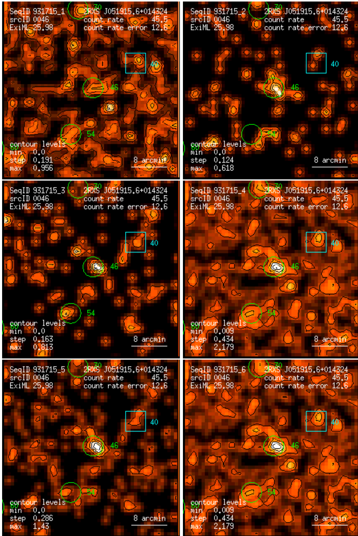
Figure 46: RASS 931715: detection 0046: band rate images, Gaussian filter: (1) PSPC channels 11 – 41, (2) 52 – 90, (3) 91 – 201, (4) 11 – 235, (5) 52 – 201, (6) 11 – 201. Broad band rates in counts/ks. Band rate contour levels in counts/ks/arcmin 2 .
