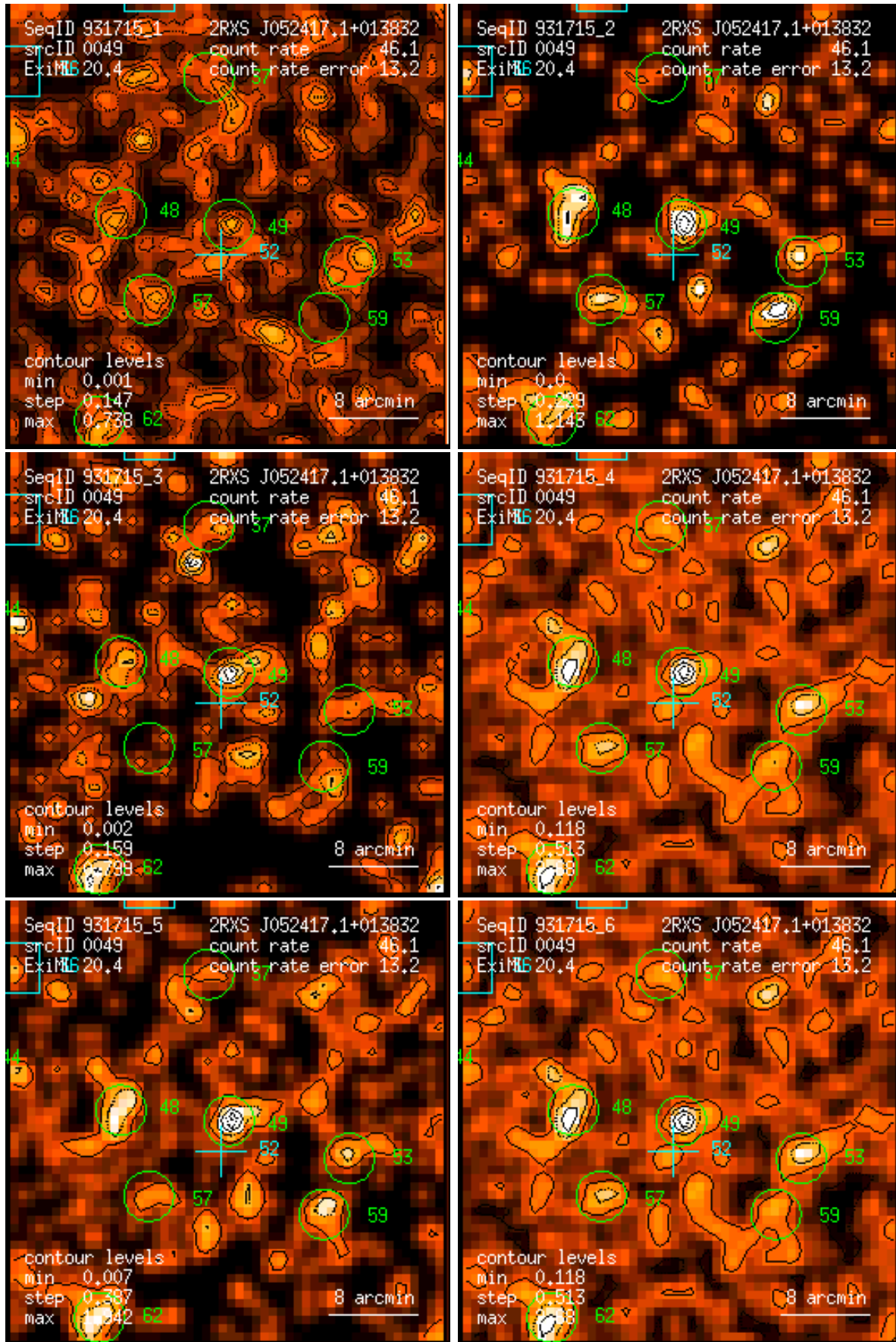
Figure 49: RASS 931715: detection 0049: band rate images, Gaussian filter: (1) PSPC channels 11 – 41, (2) 52 – 90, (3) 91 – 201, (4) 11 – 235, (5) 52 – 201, (6) 11 – 201. Broad band rates in counts/ks. Band rate contour levels in counts/ks/arcmin 2 .
