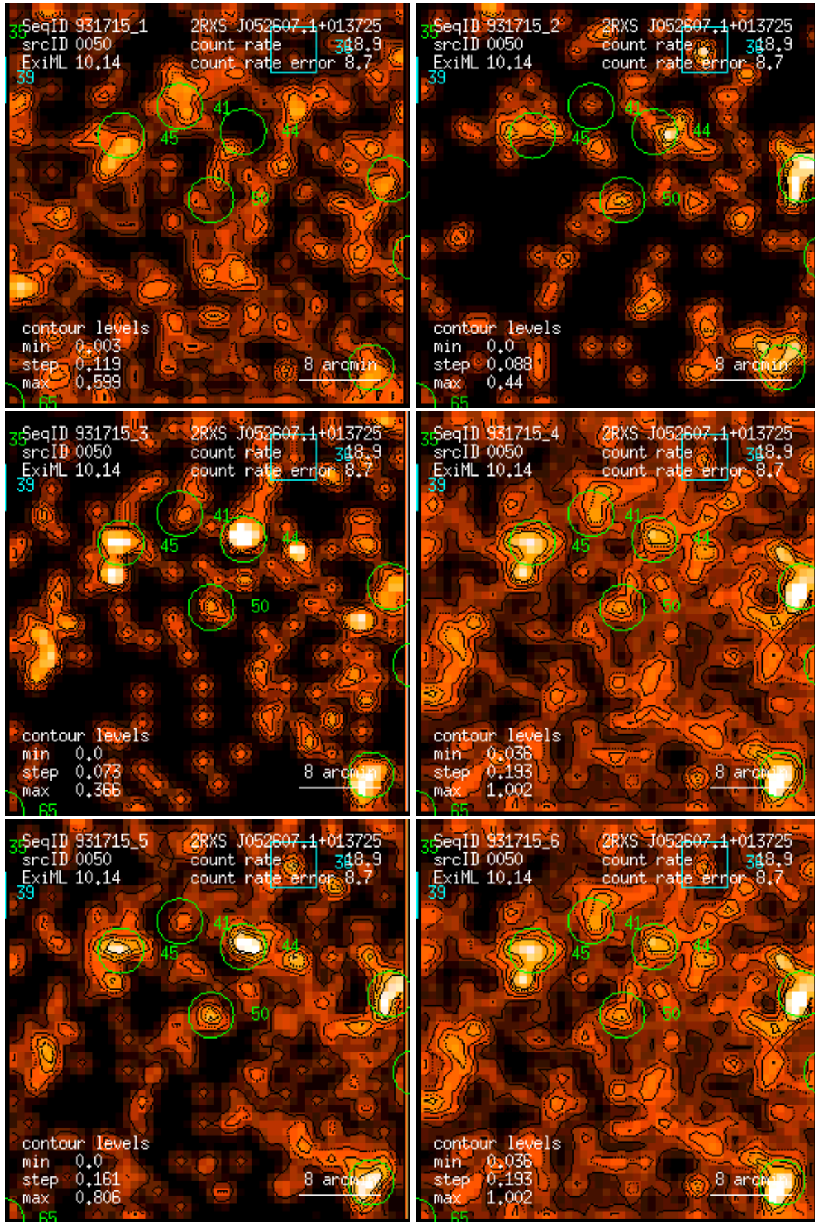
Figure 50: RASS 931715: detection 0050: band rate images, Gaussian filter: (1) PSPC channels 11 – 41, (2) 52 – 90, (3) 91 – 201, (4) 11 – 235, (5) 52 – 201, (6) 11 – 201. Broad band rates in counts/ks. Band rate contour levels in counts/ks/arcmin 2 .
