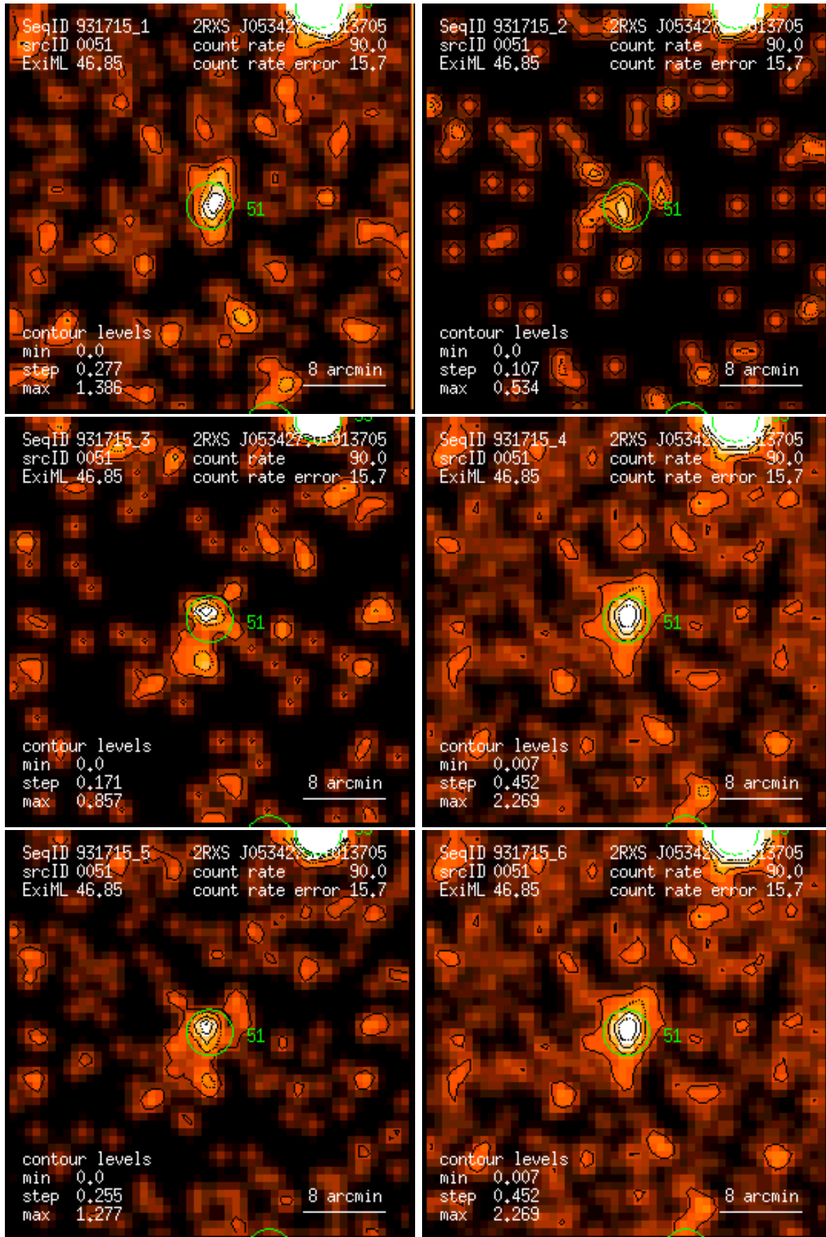
Figure 51: RASS 931715: detection 0051: band rate images, Gaussian filter: (1) PSPC channels 11 – 41, (2) 52 – 90, (3) 91 – 201, (4) 11 – 235, (5) 52 – 201, (6) 11 – 201. Broad band rates in counts/ks. Band rate contour levels in counts/ks/arcmin 2 .
