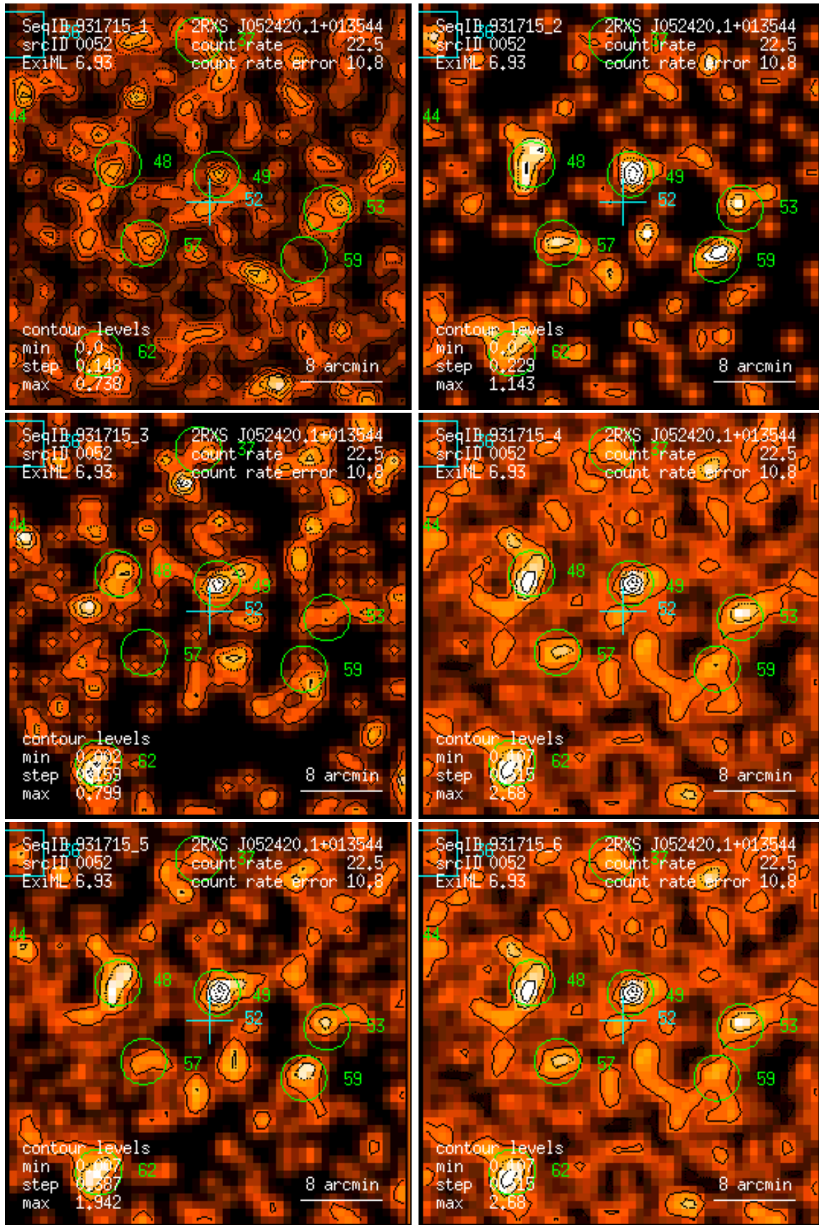
Figure 52: RASS 931715: detection 0052: band rate images, Gaussian filter: (1) PSPC channels 11 – 41, (2) 52 – 90, (3) 91 – 201, (4) 11 – 235, (5) 52 – 201, (6) 11 – 201. Broad band rates in counts/ks. Band rate contour levels in counts/ks/arcmin 2 .
