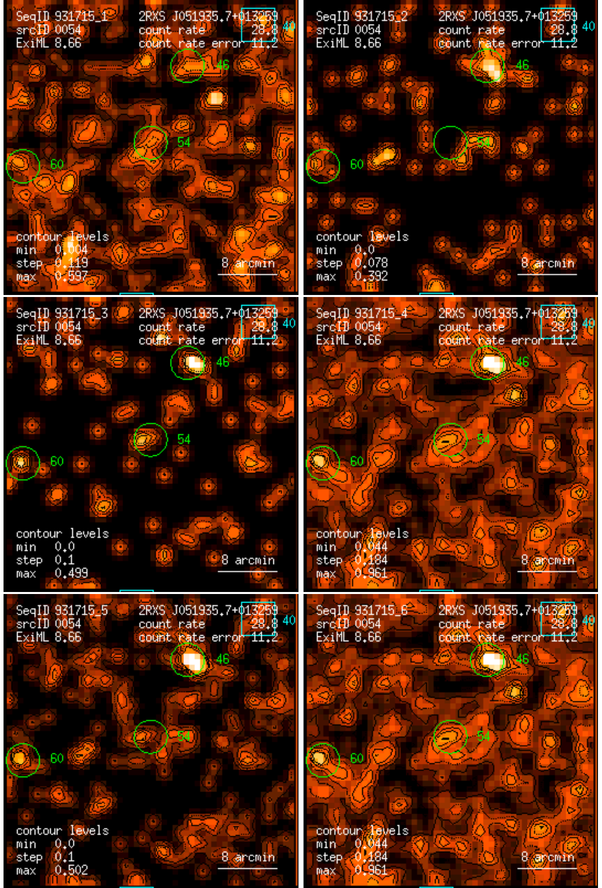
Figure 54: RASS 931715: detection 0054: band rate images, Gaussian filter: (1) PSPC channels 11 – 41, (2) 52 – 90, (3) 91 – 201, (4) 11 – 235, (5) 52 – 201, (6) 11 – 201. Broad band rates in counts/ks. Band rate contour levels in counts/ks/arcmin 2 .
