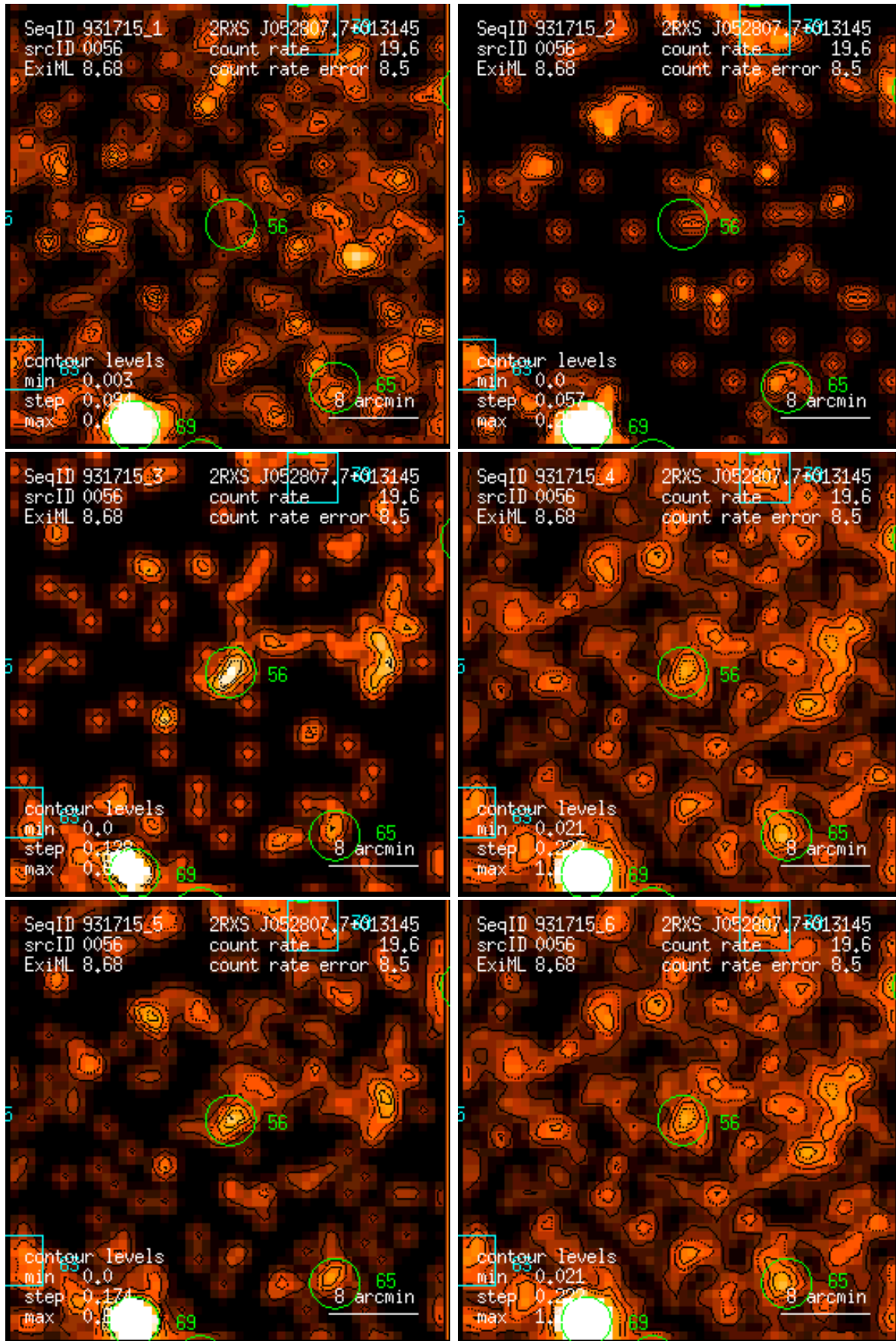
Figure 56: RASS 931715: detection 0056: band rate images, Gaussian filter: (1) PSPC channels 11 – 41, (2) 52 – 90, (3) 91 – 201, (4) 11 – 235, (5) 52 – 201, (6) 11 – 201. Broad band rates in counts/ks. Band rate contour levels in counts/ks/arcmin 2 .
