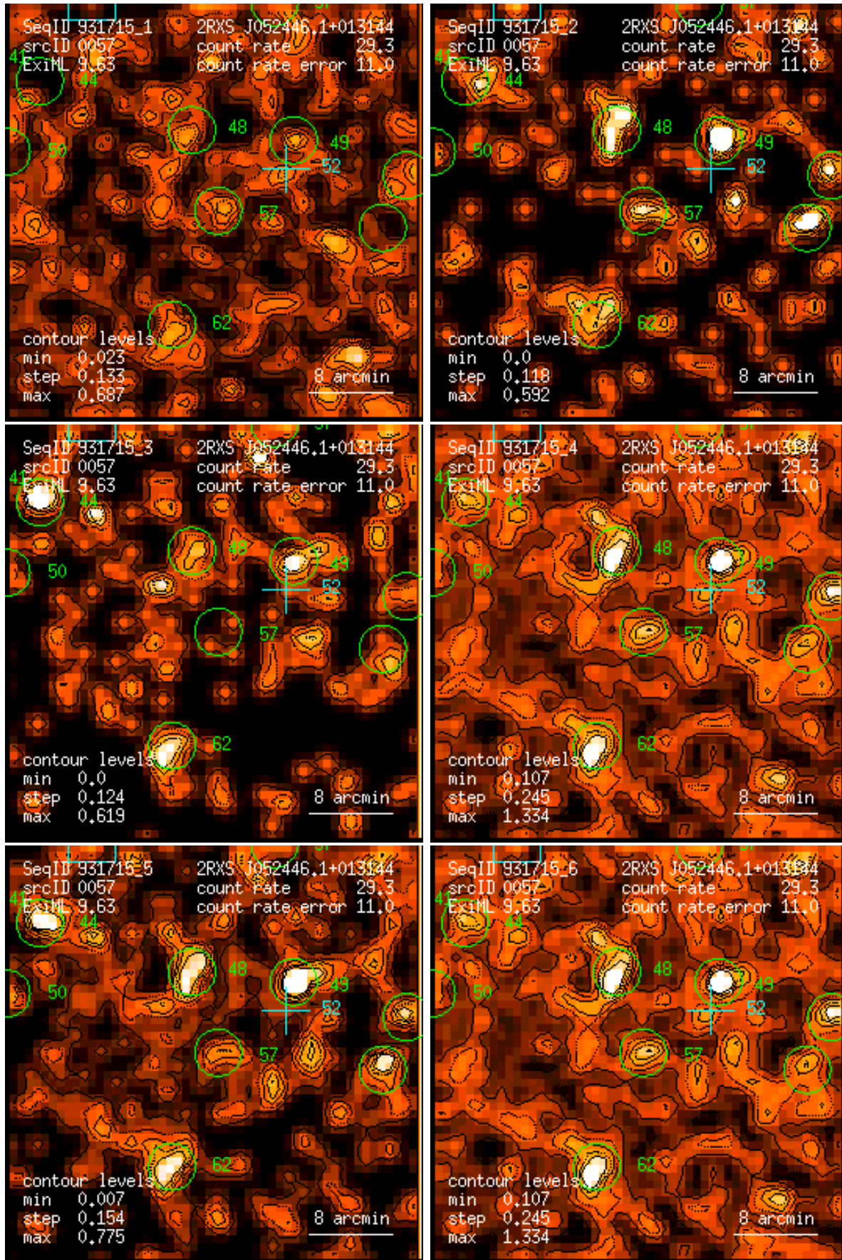
Figure 57: RASS 931715: detection 0057: band rate images, Gaussian filter: (1) PSPC channels 11 – 41, (2) 52 – 90, (3) 91 – 201, (4) 11 – 235, (5) 52 – 201, (6) 11 – 201. Broad band rates in counts/ks. Band rate contour levels in counts/ks/arcmin 2 .
