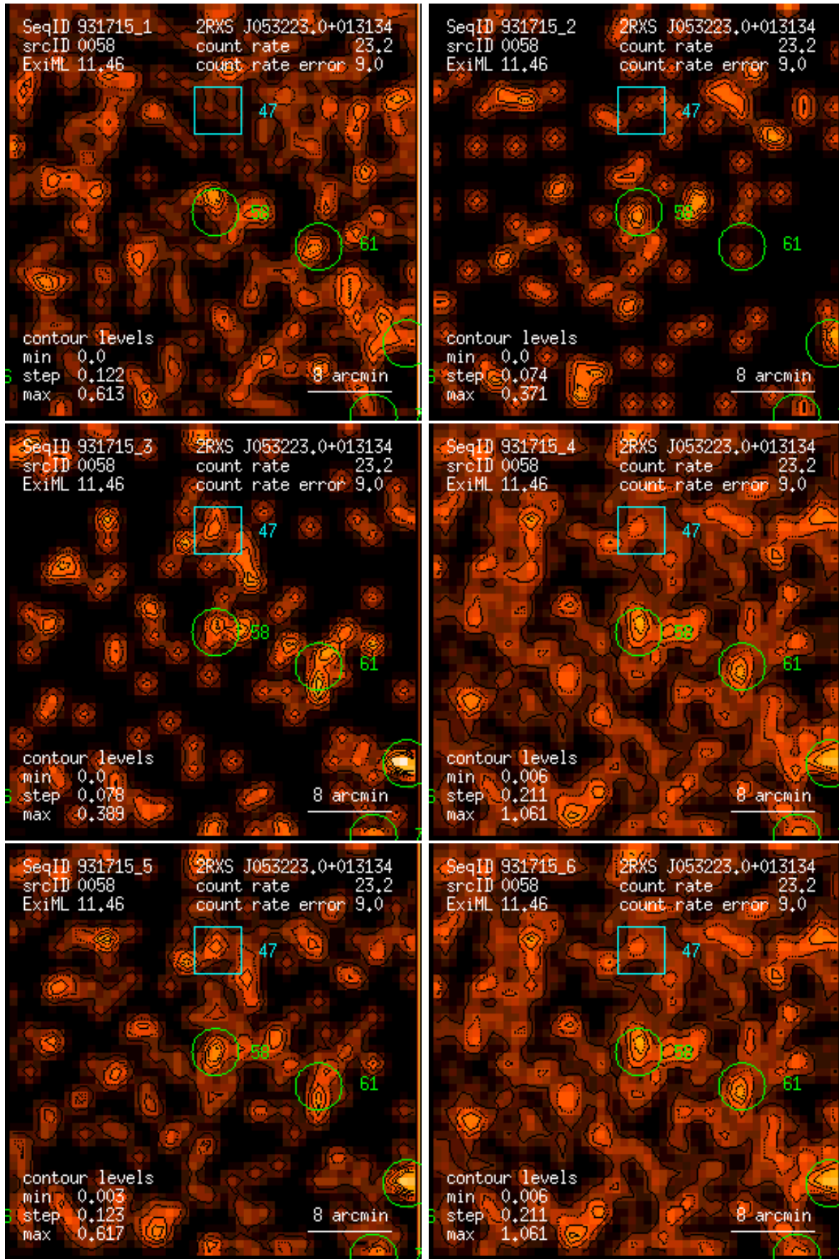
Figure 58: RASS 931715: detection 0058: band rate images, Gaussian filter: (1) PSPC channels 11 – 41, (2) 52 – 90, (3) 91 – 201, (4) 11 – 235, (5) 52 – 201, (6) 11 – 201. Broad band rates in counts/ks. Band rate contour levels in counts/ks/arcmin 2 .
