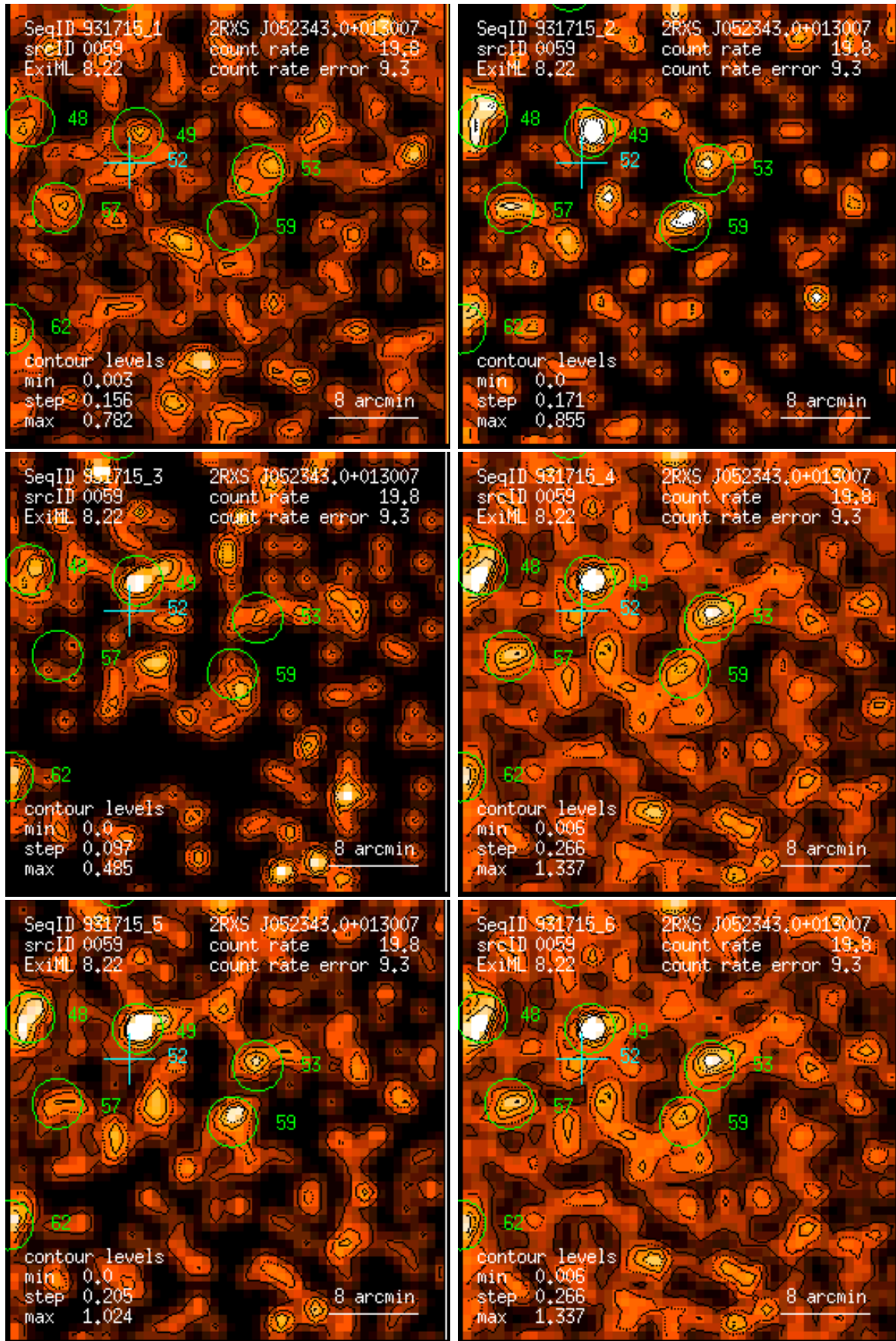
Figure 59: RASS 931715: detection 0059: band rate images, Gaussian filter: (1) PSPC channels 11 – 41, (2) 52 – 90, (3) 91 – 201, (4) 11 – 235, (5) 52 – 201, (6) 11 – 201. Broad band rates in counts/ks. Band rate contour levels in counts/ks/arcmin 2 .
