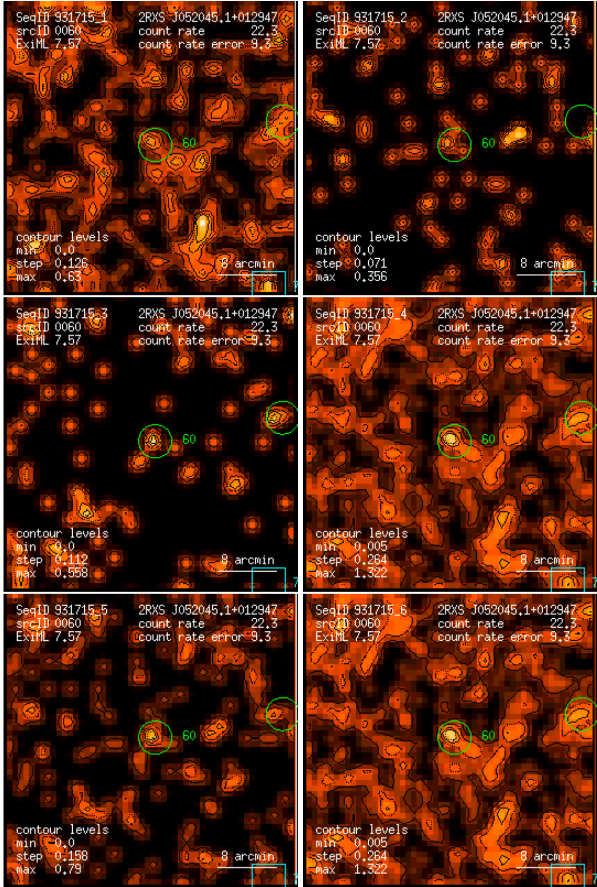
Figure 60: RASS 931715: detection 0060: band rate images, Gaussian filter: (1) PSPC channels 11 – 41, (2) 52 – 90, (3) 91 – 201, (4) 11 – 235, (5) 52 – 201, (6) 11 – 201. Broad band rates in counts/ks. Band rate contour levels in counts/ks/arcmin 2 .
